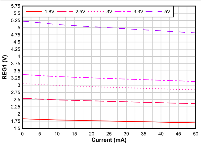
6-13. REG1 Voltage vs. Load at 25°C
