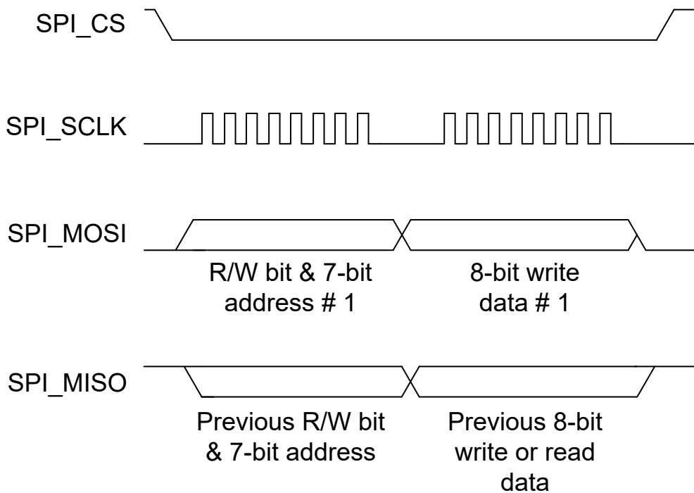
図 7-15. SPI Transaction #1 Without CRC
