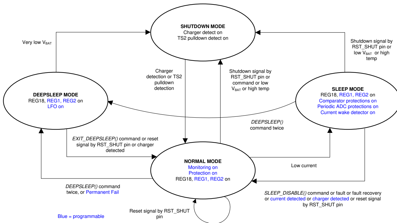
7-7. Device Functional Modes
