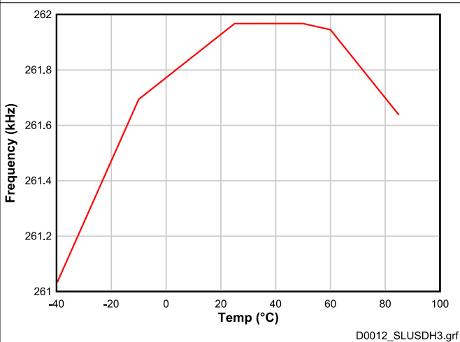
図 6-7. Low Frequency Oscillator (LFO) Accuracy vs. Temperature
