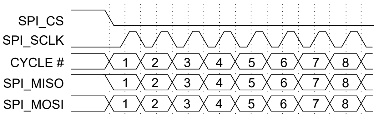
図 7-11. SPI with CPOL = 0 and CPHA = 0
