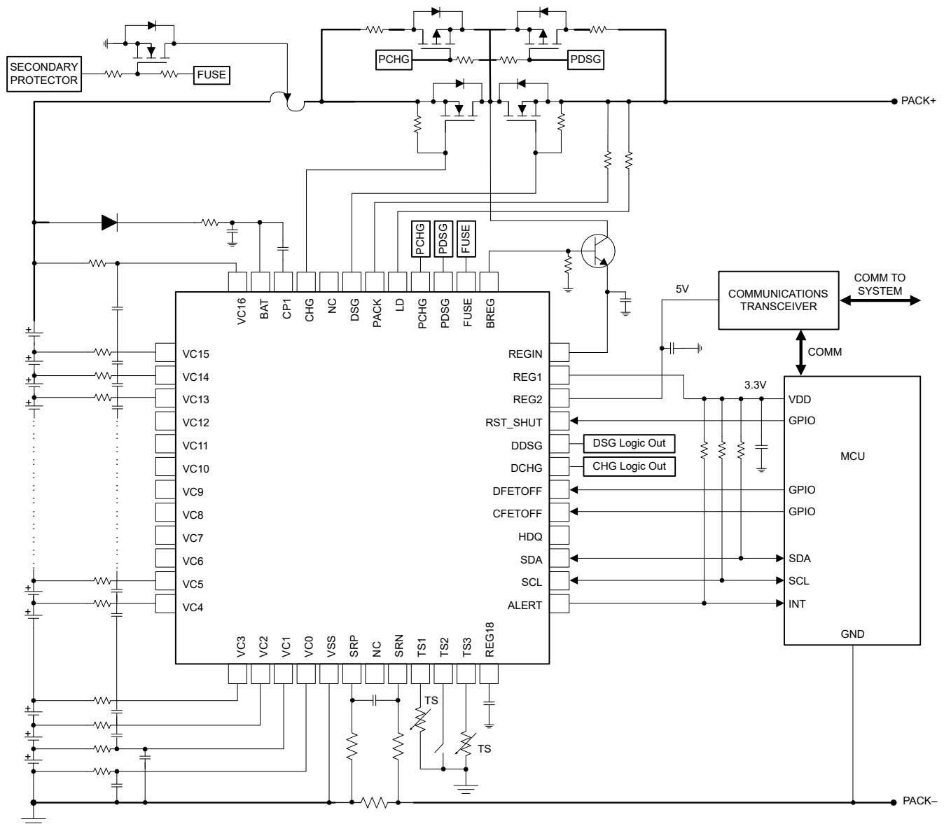
8-1. BQ76972 16-Series Cell Typical Implementation (Simplified Schematic)
