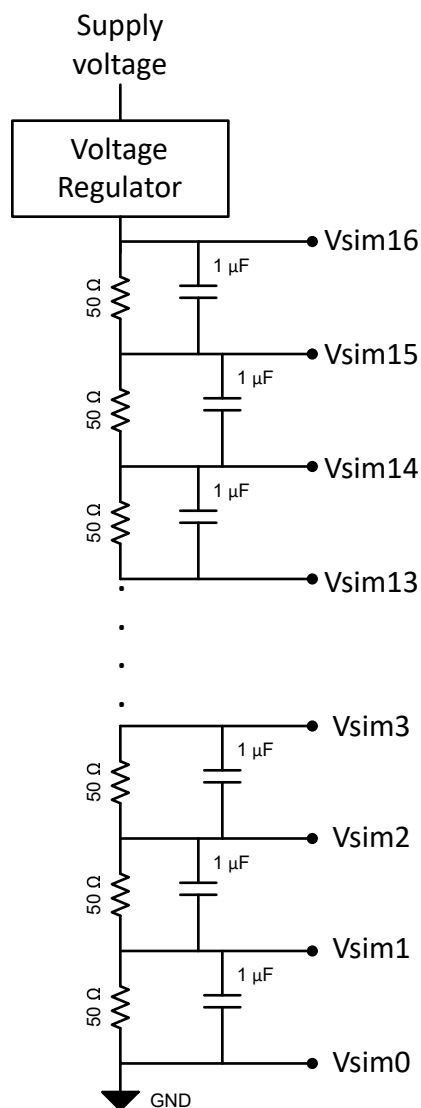
図 7-4. Example Fixture for Cell Offset Calibration
