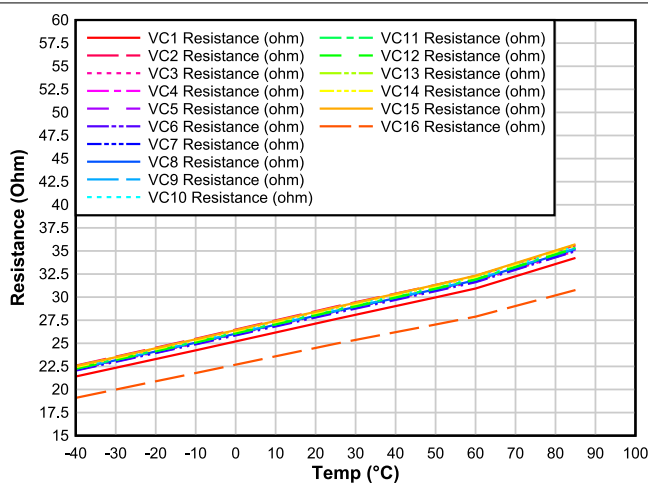
6-11. Cell Balancing Resistance vs. Temperature
