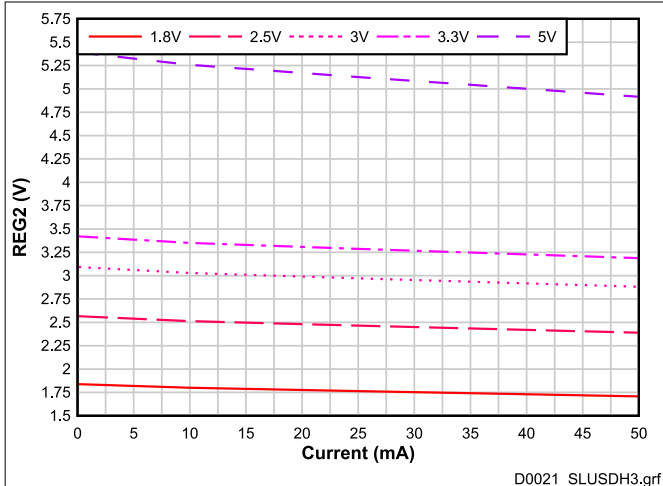
図 6-14. REG2 Voltage vs. Load at 25°C
