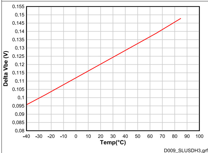
図 6-6. Internal Temperature Sensor (Delta V_{BE} ) Voltage vs. Temperature
