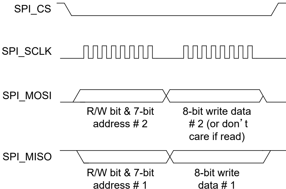
図 7-16. SPI Transaction #2 Without CRC
