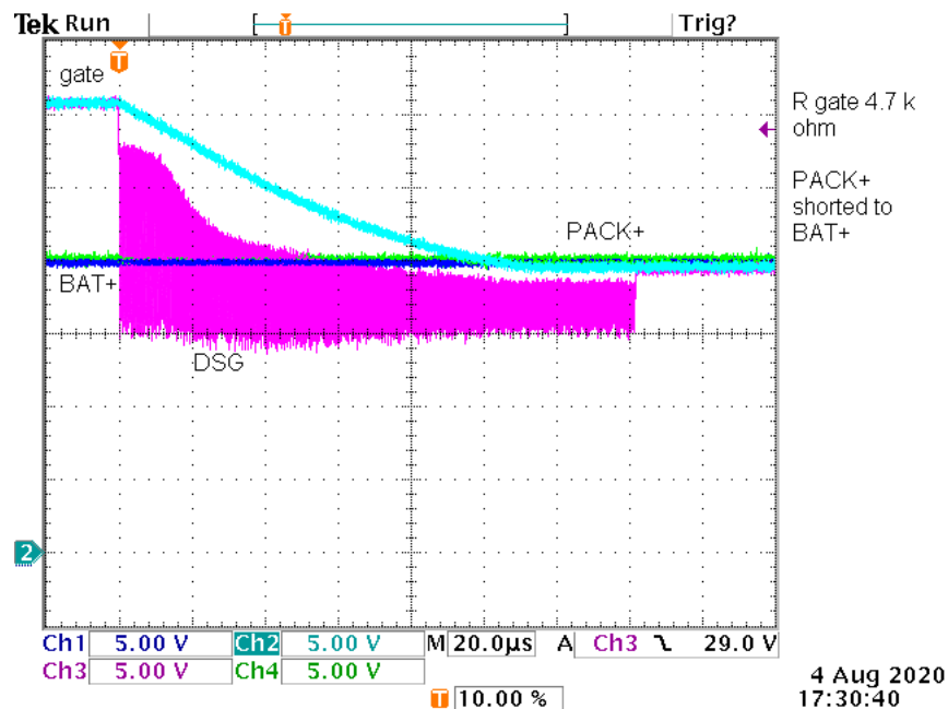
図 8-8. A Slower Turn-Off Case Using a 4.7-kΩ Series Gate Resistor, and the PACK+ Connector Shorted to the Top of the Stack
