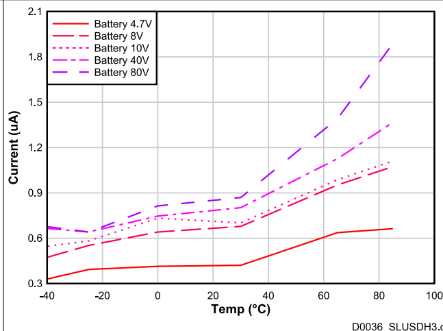
6-23. BAT Current in SHUTDOWN Mode vs. Temperature
