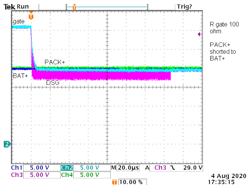
図 8-9. A Fast Turn-Off Case with a 100-Ω Series Gate Resistor
