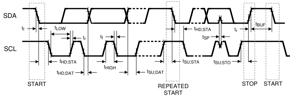
図 6-1. I²C Communications Interface Timing
