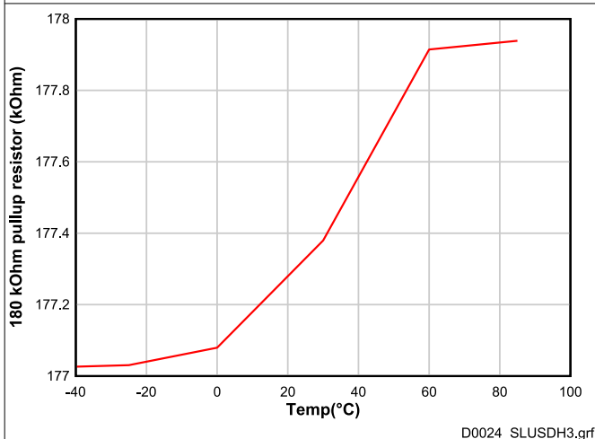
図 6-16. Thermistor Pullup Resistance vs. Temperature (180-kΩ Setting)
