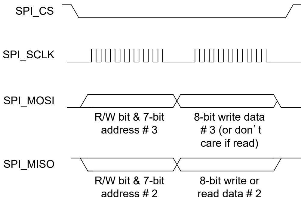
✎ 7-17. SPI Transaction #3 Without CRC
