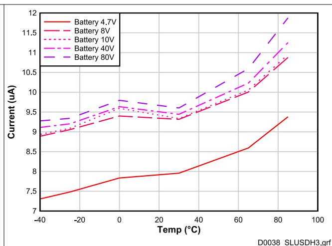
6-25. BAT Current in DEEPSLEEP2 (No LFO) Mode vs. Temperature
