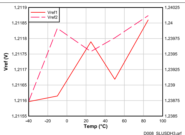
図 6-5. Internal Voltage References vs. Temperature (VREF1 and VREF2)
