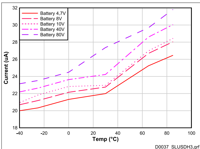
6-24. BAT Current in SLEEP2 (SRC Follower) Mode vs. Temperature
