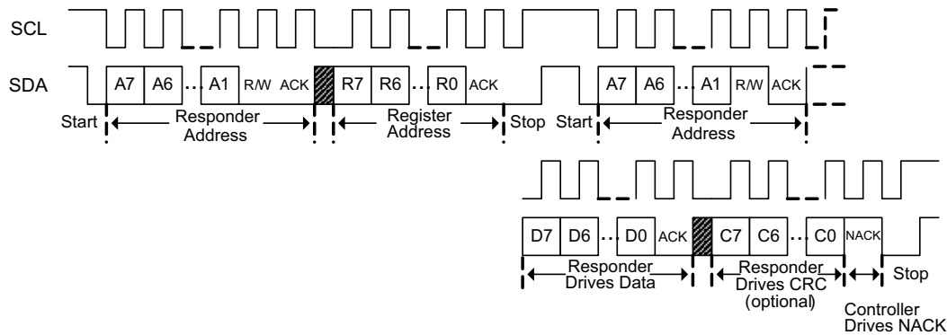
図 7-10. I²C Read Without Repeated Start
