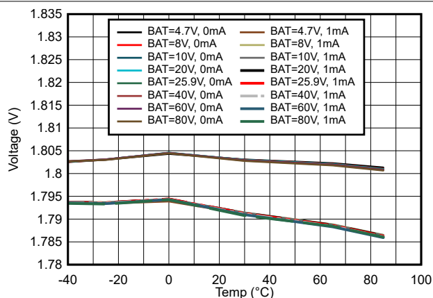
6-20. REG18 Voltage vs. Temperature, Across BAT Levels
