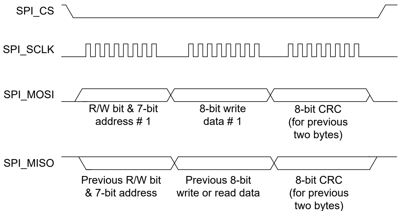
図 7-12. SPI Transaction #1 Using CRC
