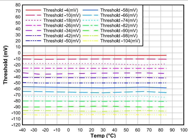
6-9. Overcurrent in Discharge Protection 1 (OCD1) Threshold vs. Temperature
