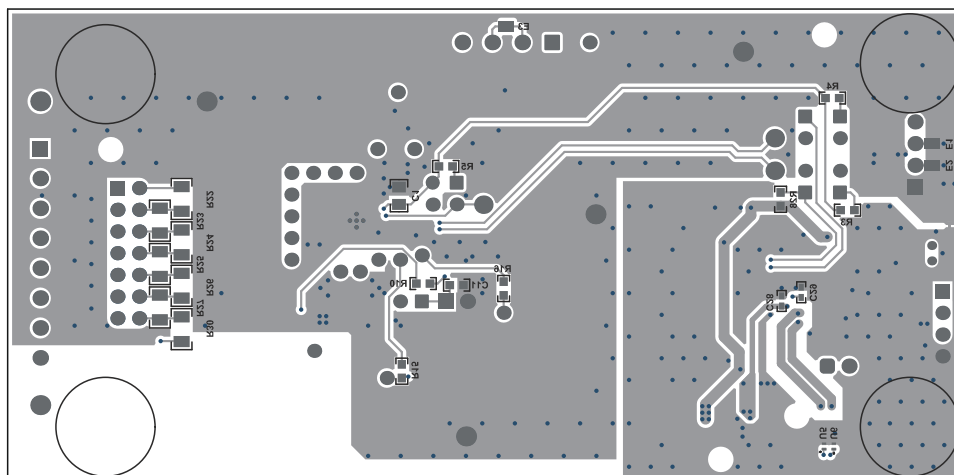
図 10-2. BQ77307 Two-Layer Board Layout—Bottom Layer
