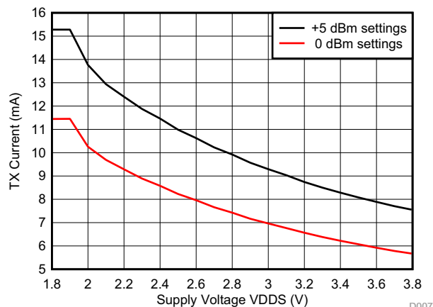
7-10. TX Current Consumption vs Supply Voltage (VDD5)
