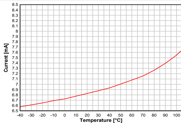
図 8-6. RX Current vs. Temperature (BLE 1 Mbps, 2.44 GHz)
