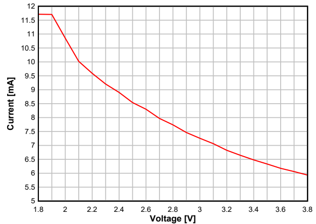
図 8-9. TX Current vs. Supply Voltage (VDD) (BLE 1 Mbps, 2.44 GHz, 0 dBm)
