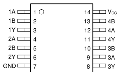
図 3-1. CD54AC00 J Package, 14-Pin CDIP; CD74AC00 D or N Packages, 14-Pin SOIC, or PDIP (Top View)
