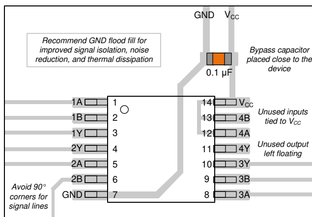
11-1. Example layout for the CD74HC7266
