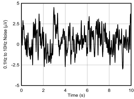
图 5-51. Internal Reference Noise
