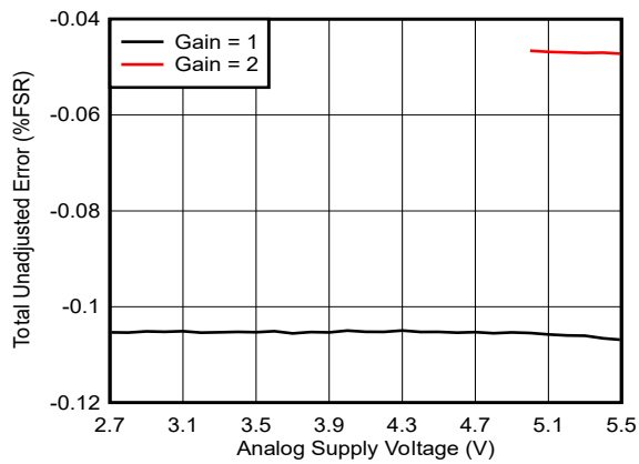
5-15. Total Unadjusted Error vs Supply Voltage
