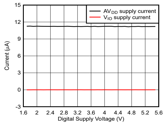
5-28. Power-Down Current vs V_{IO}
