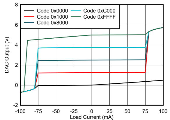
5-30. Headroom vs Load Current
