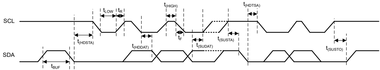
図 5-1. I 2 C Timing Diagram
