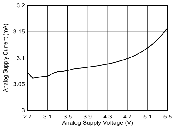
5-25. Supply Current With Internal Reference vs Supply Voltage
