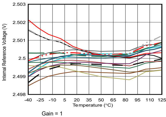
5-47. Internal Reference Voltage vs Temperature
