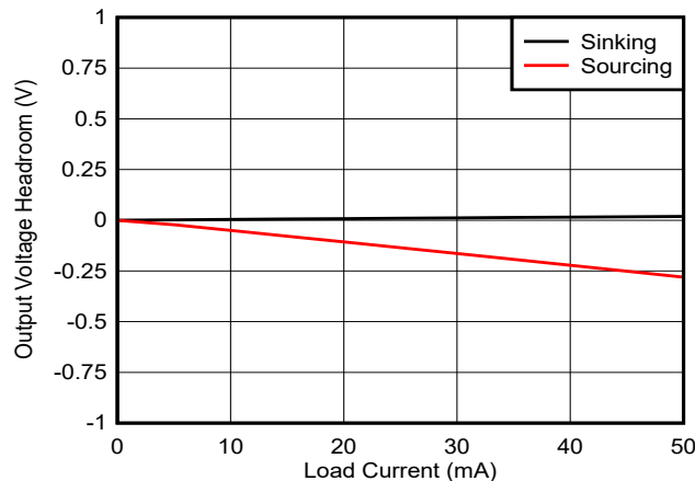
☒ 8-3. Headroom vs Load Current
