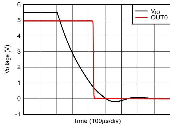
图 5-40. V_{IO} Power Down Response
