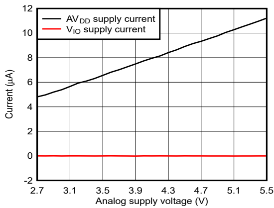
5-27. Power-Down Current vs Supply Voltage
