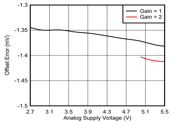
5-16. Offset Error vs Supply Voltage
