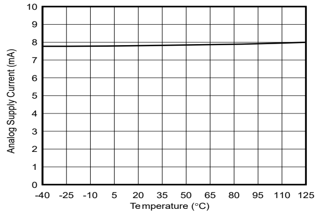
5-22. Supply Current With External Reference vs Temperature
