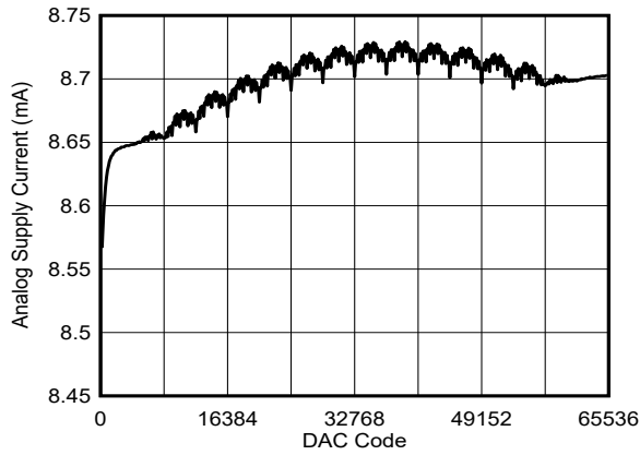
5-21. Supply Current With Internal Reference vs Digital Input Code
