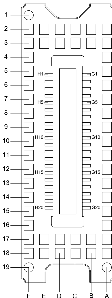
図 5-1. FQJ Package 40-Pin Connector Bottom View
