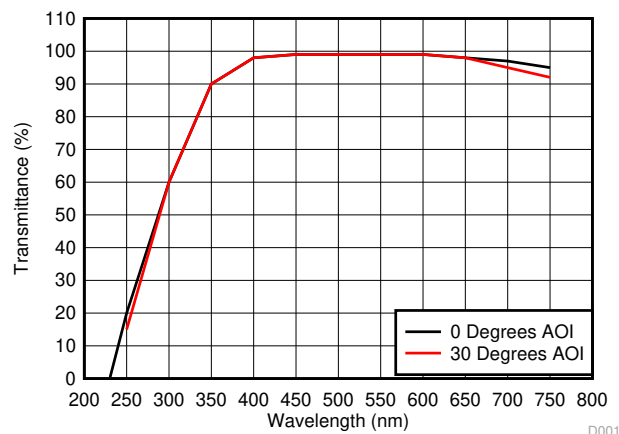
FIG 7-6. DLP4500 DMD Window Transmittance
