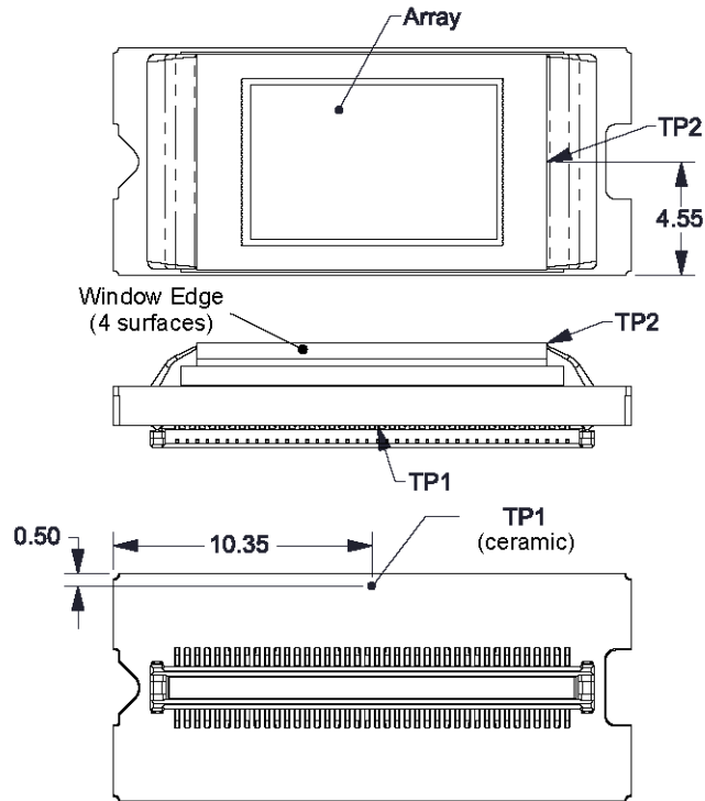
図 8-3. Thermal Test Point Location - FQE Package
