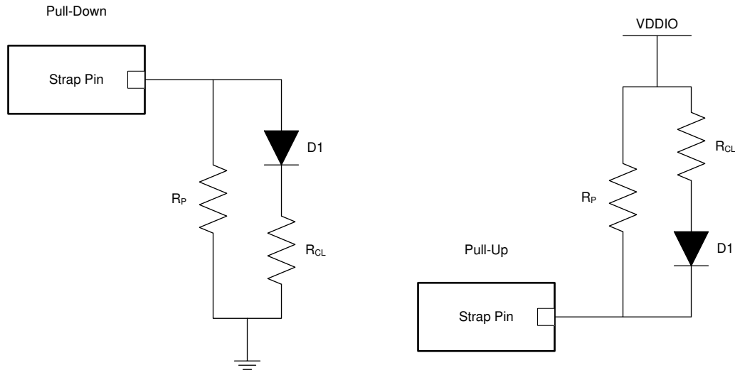
図 7-19. Example Strap Connections
