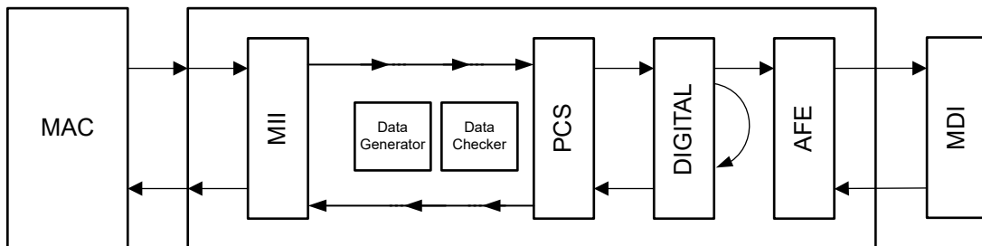
図 7-6. Digital loopback without data generator
