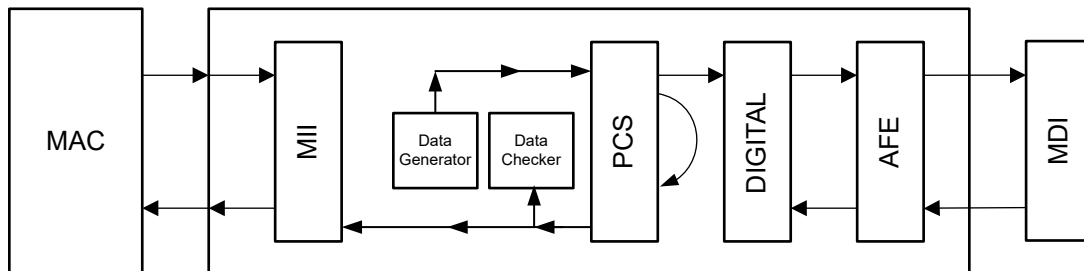
図 7-3. PCS Loopback with data generator
