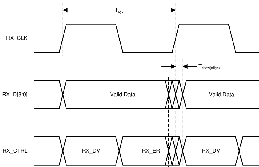
図 6-5. RGMII Receive Timing (Internal Delay Disabled)
