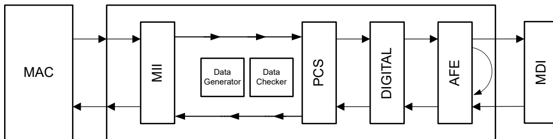
図 7-8. Analog loopback without data generator
