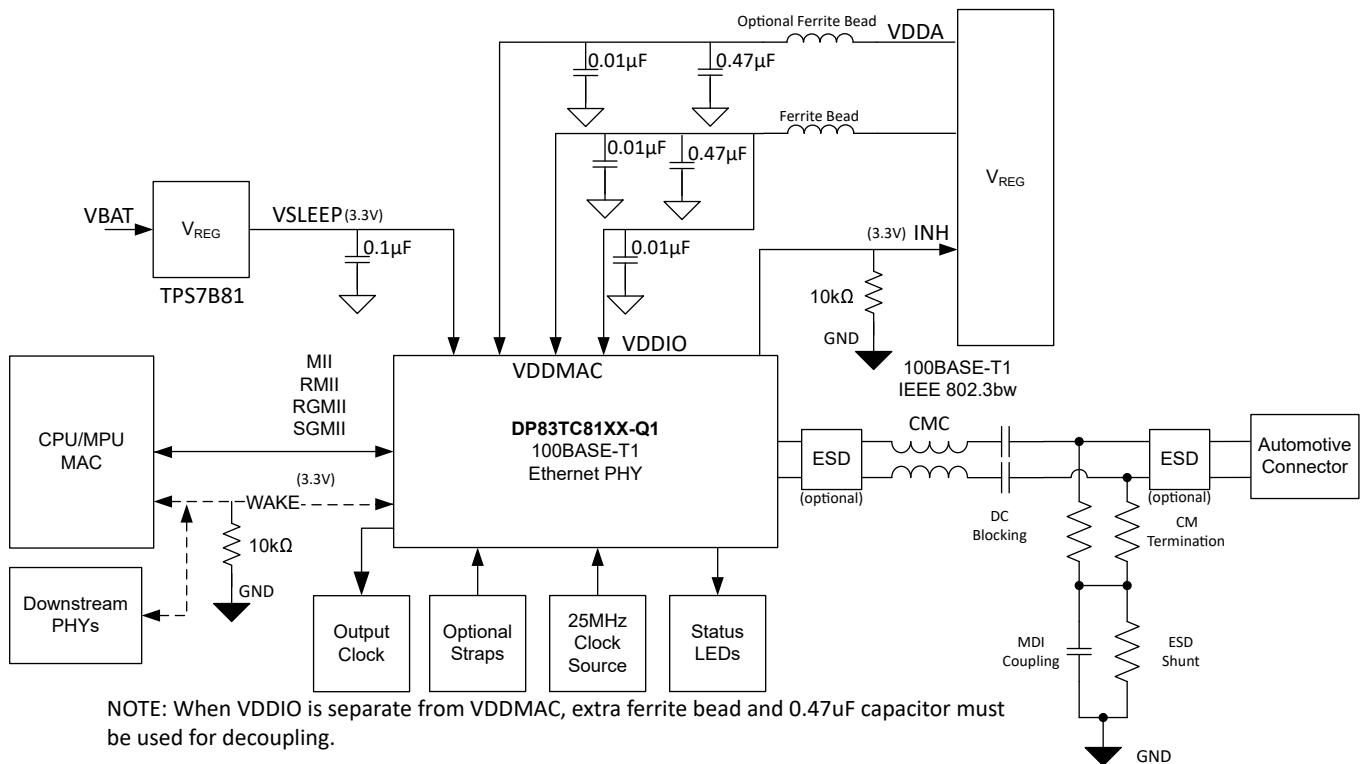
8-9. Typical TC-10 Application With Peripherals
