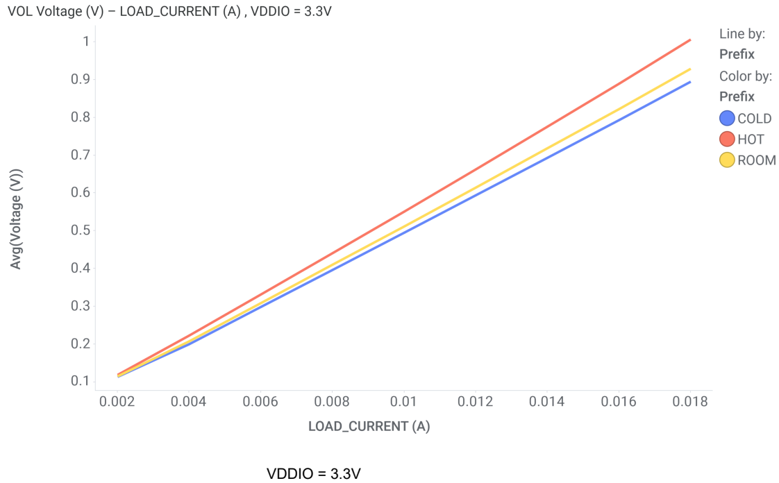
図 6-12. LED pins VOL (3.3V)
