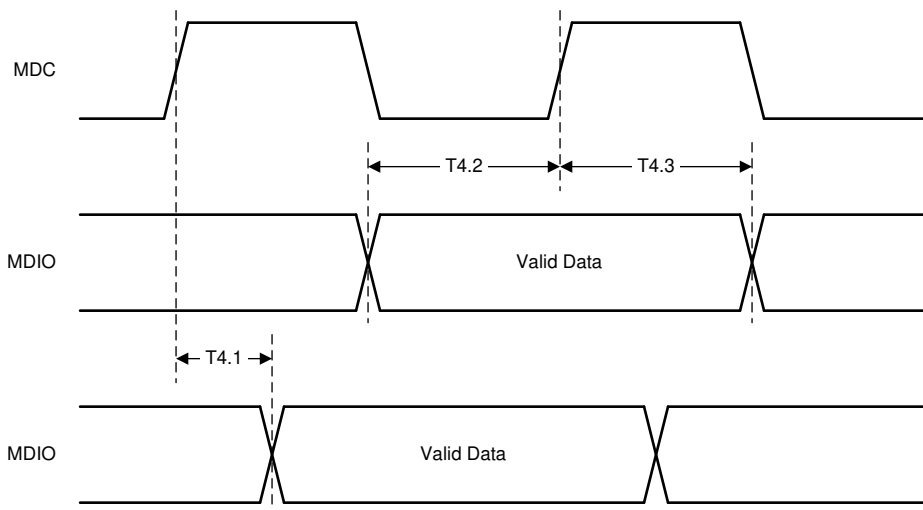
図 6-6. Serial Management Timing
