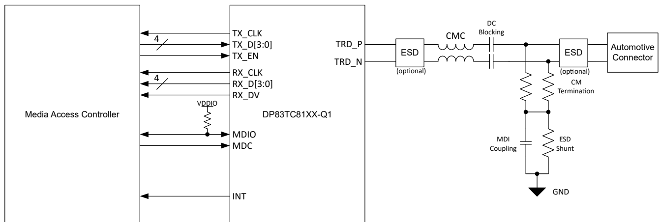
図 8-2. Typical Application (MII)
