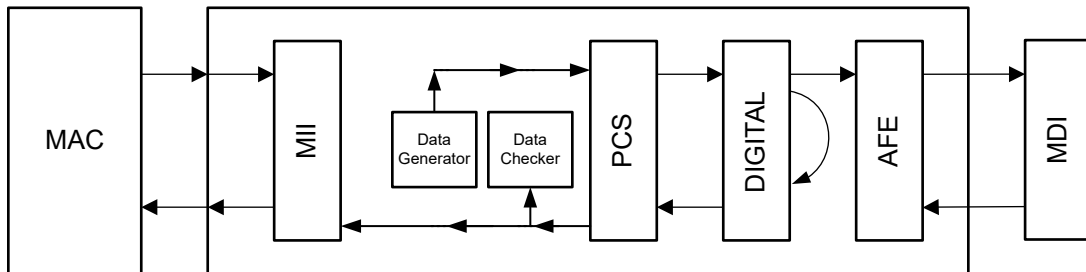
図 7-5. Digital loopback with data generator
