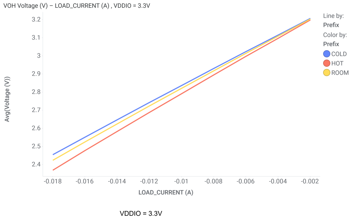
図 6-13. LED pins VOH (3.3V)
