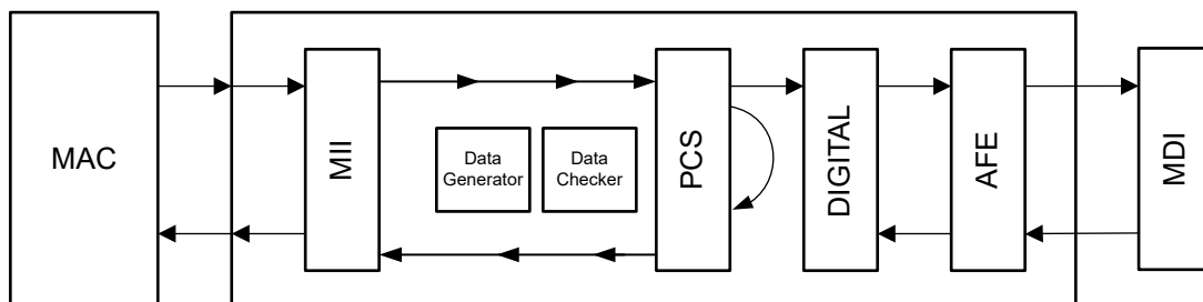
図 7-4. PCS Loopback without data generator
