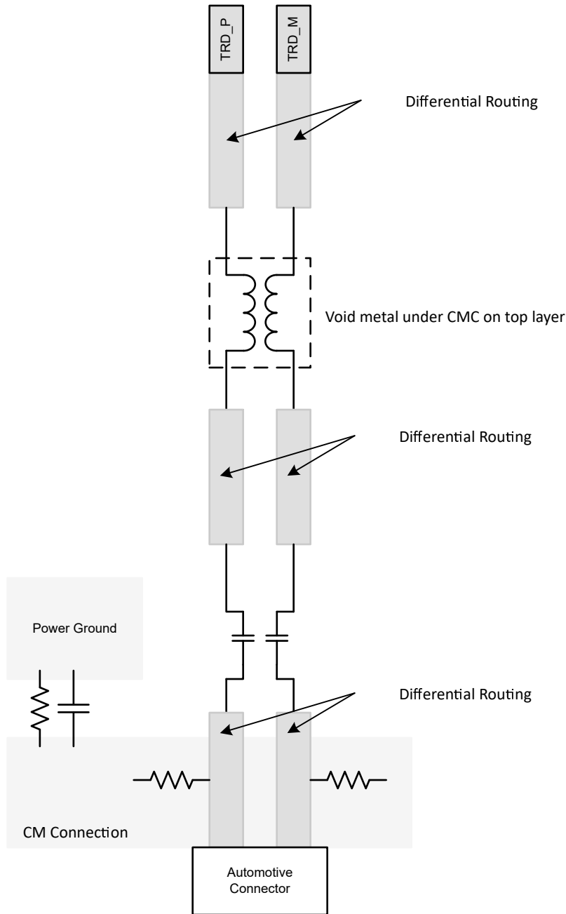
図 8-13. MDI Low-Pass Filter Layout Recommendation
