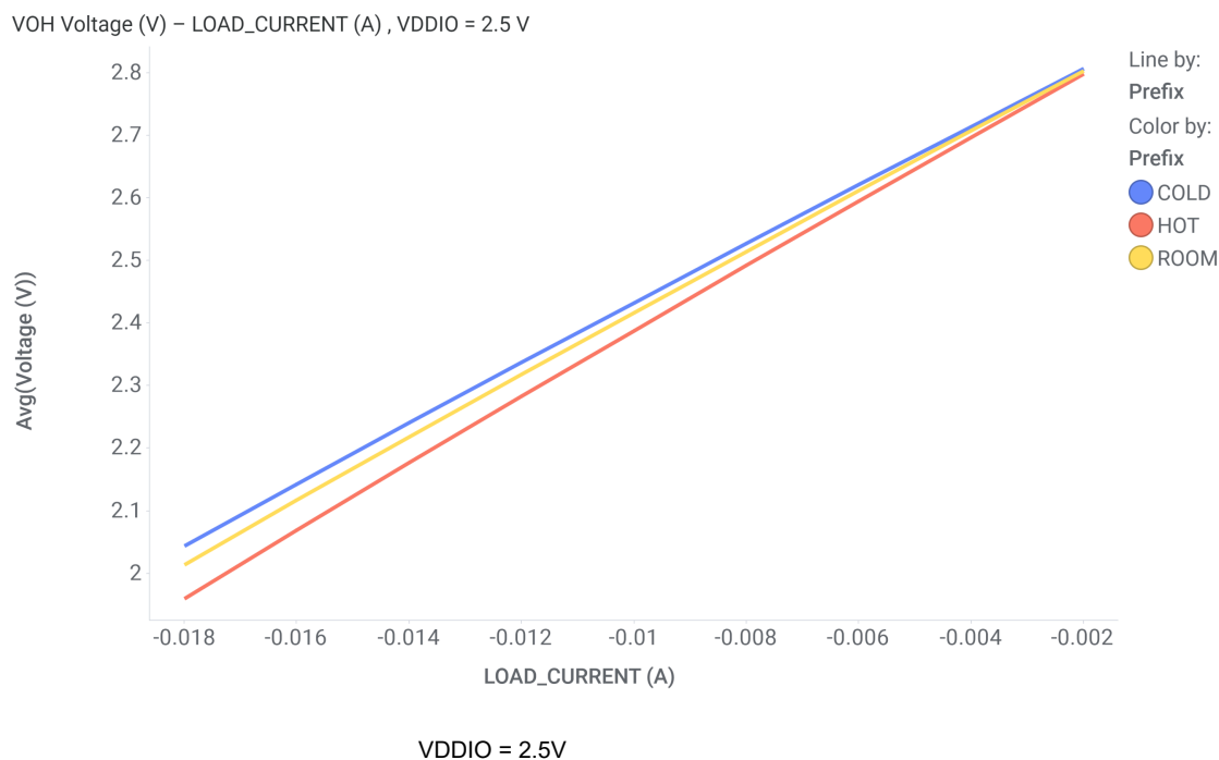
図 6-11. LED pins VOH (2.5V)
