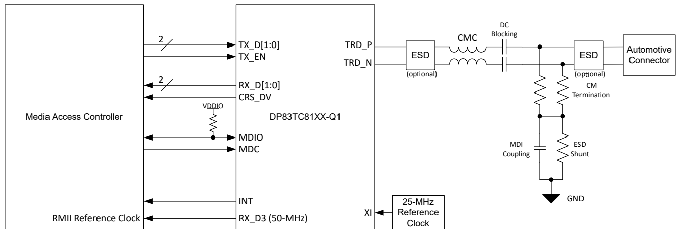
8-4. Typical Application (RMII Master)
