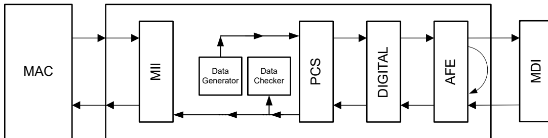
図 7-7. Analog loopback with data generator
