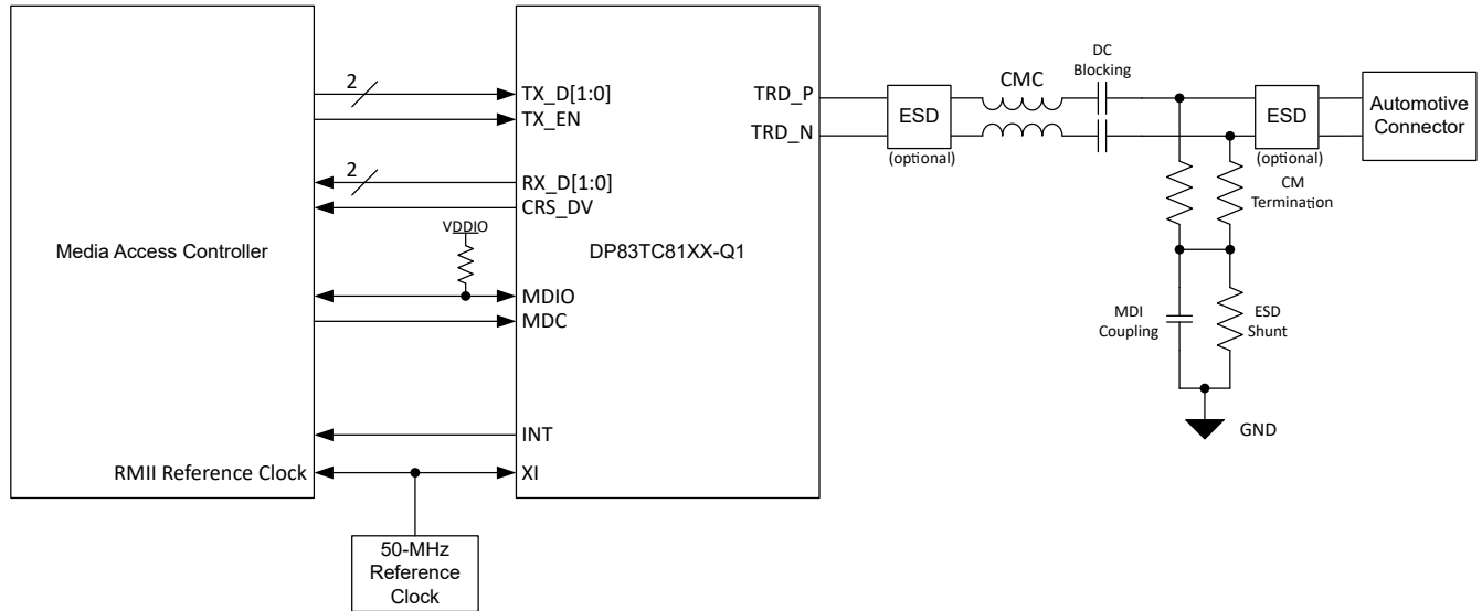
8-3. Typical Application (RMII Slave)
