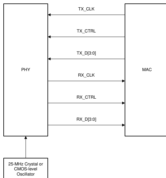
図 7-16. RGMII Connections
