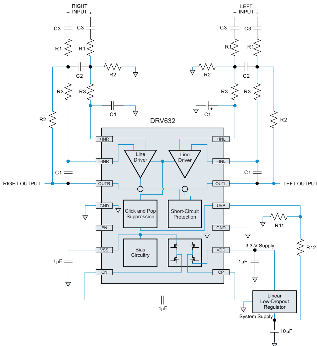
Figure 9. Typical Application Schematic
