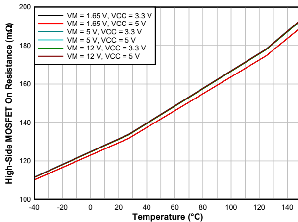
図 7-3. High-Side MOSFET On Resistance (mΩ)
