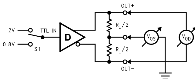
7-1. Differential Driver DC Test Circuit
