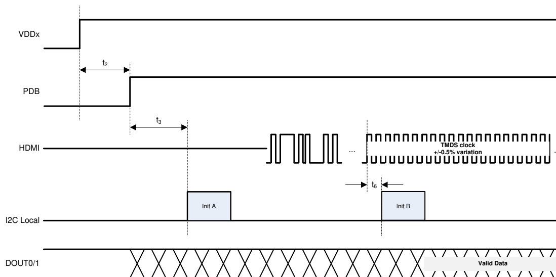
Figure 33. Initialization Sequencing
