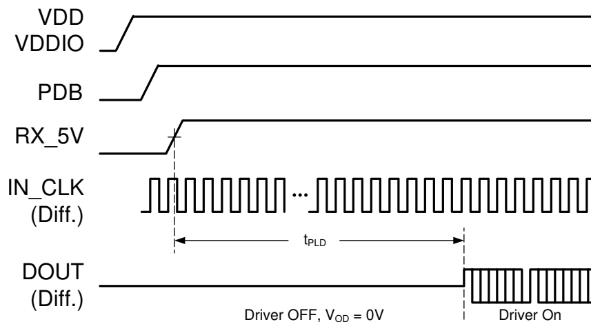
FIG 3. Serializer Lock Time
