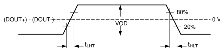
FIG 2. Output Transition Times
