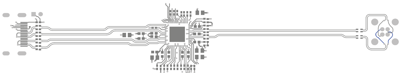
✎ 34. DS90UB949A-Q1 Serializer Layout Example
