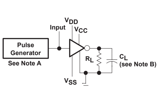
TEST CIRCUIT
