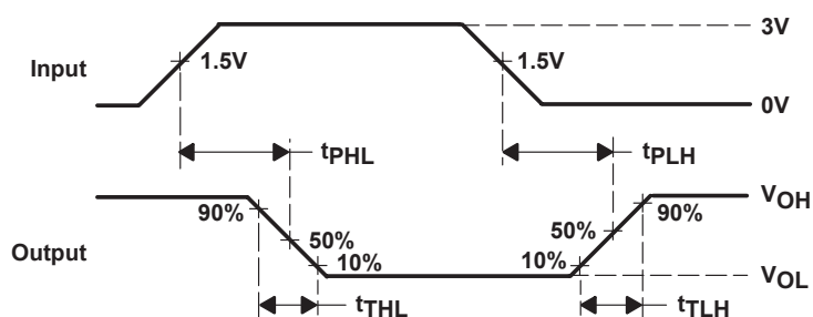
VOLTAGE WAVEFORMS
