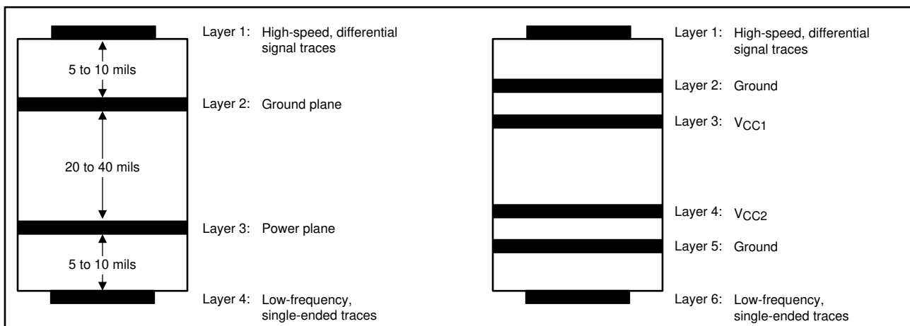
FIG 10-1. Recommended 4- or 6- Layer (0.062") Stack for a Receiver PCB Design
