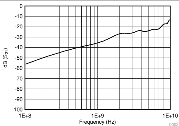
6-3. Off Isolation
