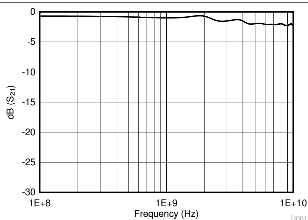
6-1. Insertion Loss and -3 dB Bandwidth
