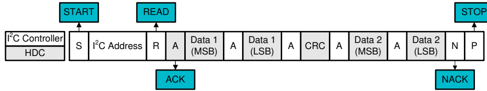
Figure 8-7. I 2 C Read Multi Data Result, Final CRC Discarded
