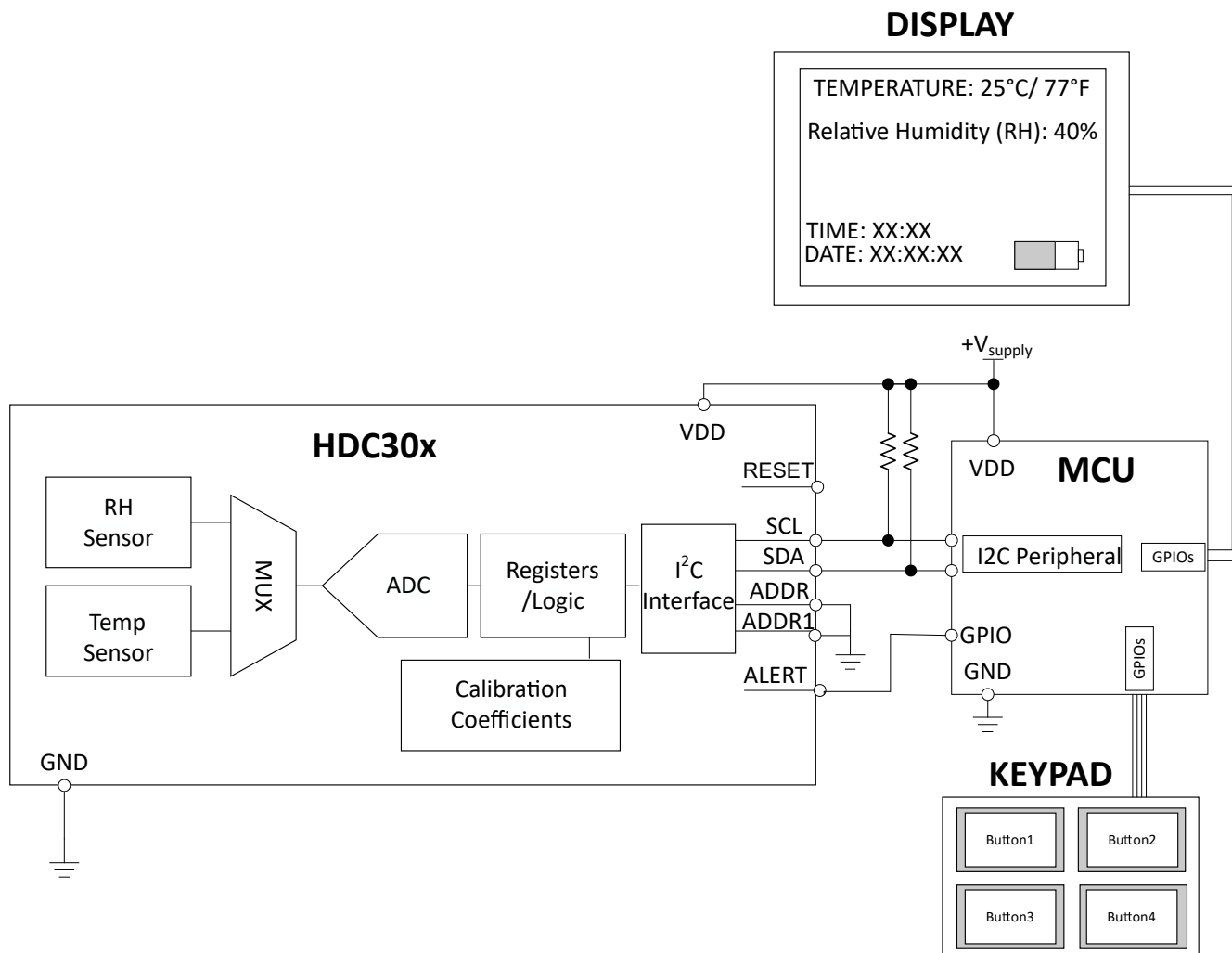
9-1. Typical Application Schematic HVAC
