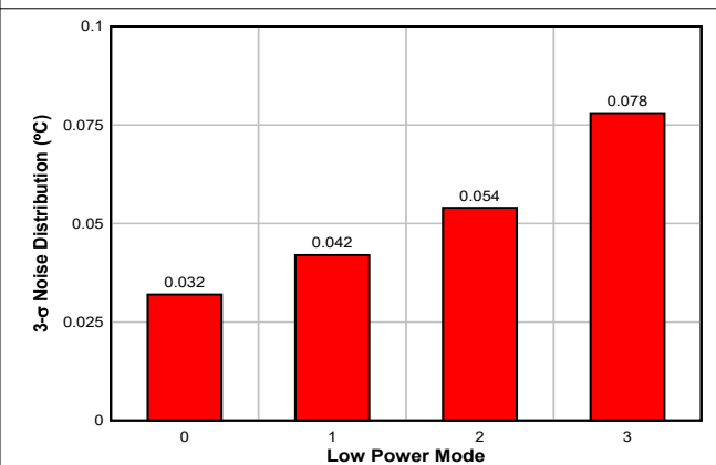
Figure 7-7. Typical Temperature Noise Across Low Power Modes
