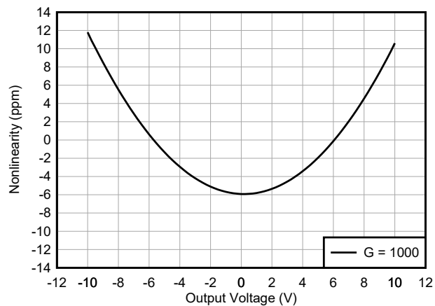
FIG 7-40. Gain Nonlinearity
