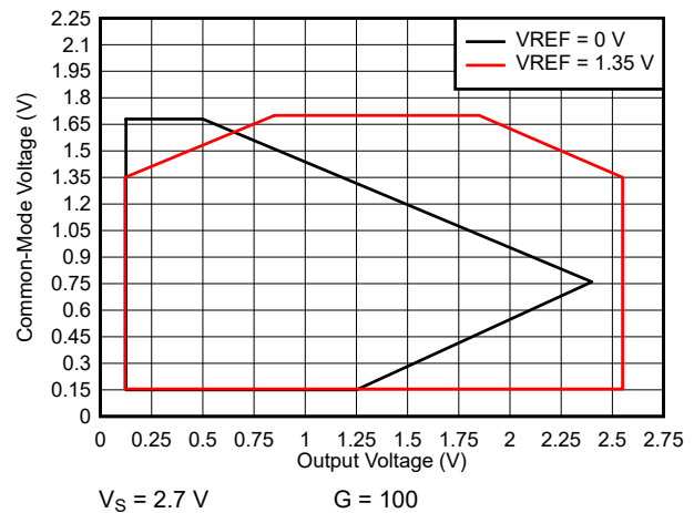
7-54. Input Common-Mode Voltage vs Output Voltage
