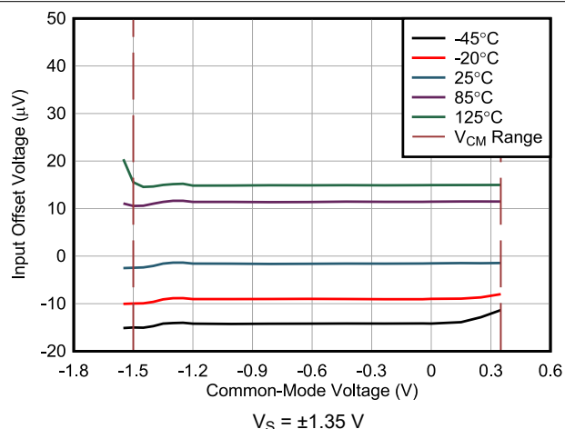
7-48. Offset Voltage vs Common-Mode Voltage
