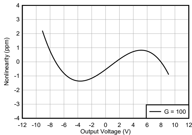
FIG 7-39. Gain Nonlinearity
