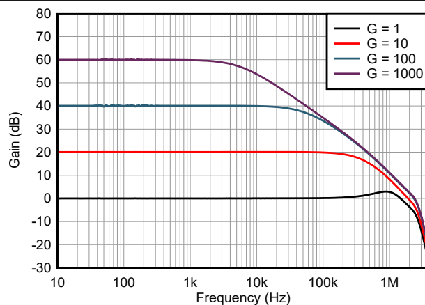
7-20. Closed-Loop Gain vs Frequency
