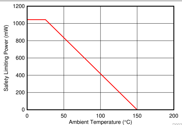
6-2. Thermal Derating Curve for Limiting Power per VDE for 8-D Package
