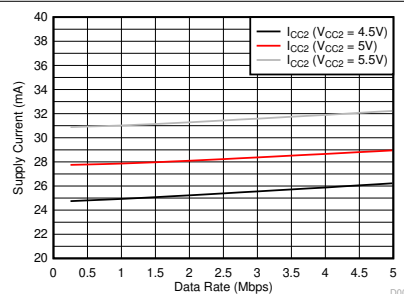
6-4. Side 2 Supply Current vs Datarate
