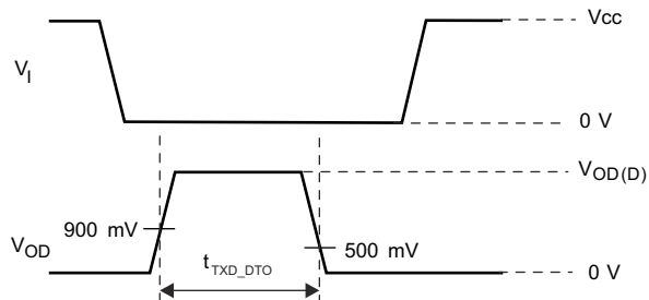
7-7. Dominant Time-out Test Circuit and Voltage Waveforms
