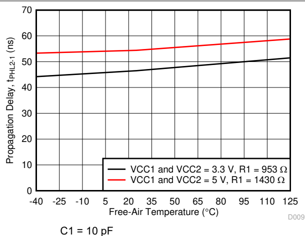
6-12. t_{PLH2-1} Propagation Delay vs Free-Air Temperature
