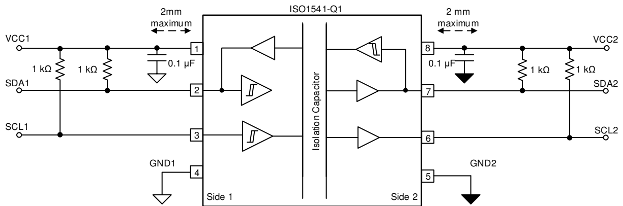
8-6. Typical ISO1541-Q1 Circuit Hookup
