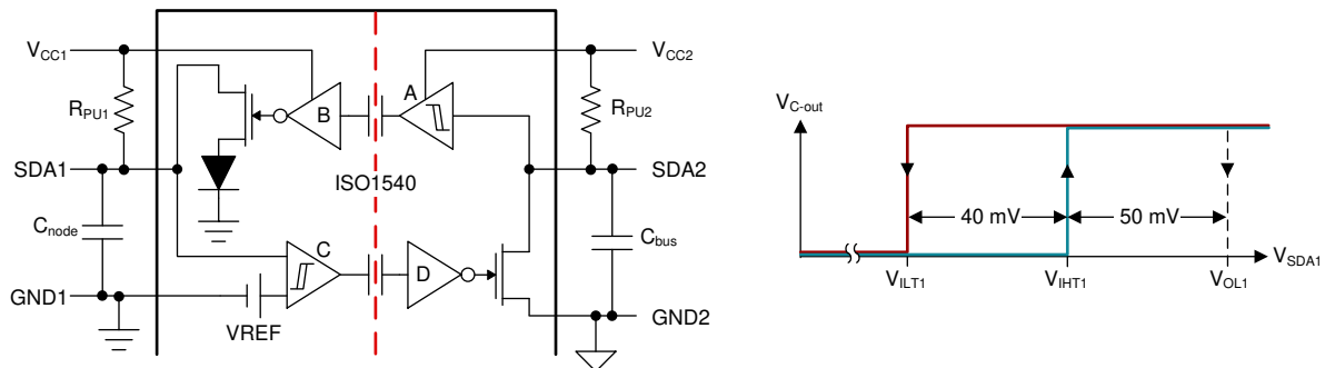
図 7-3. SDA Channel Design and Voltage Levels at SDA1
