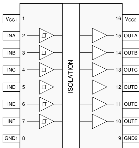
図 5-1. ISO7760-Q1 DW and DBQ Packages 16-Pin SOIC and SSOP Top View
