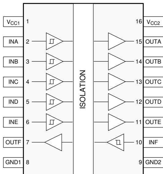
図 5-2. ISO7761-Q1 DW and DBQ Packages 16-Pin SOIC and SSOP Top View
