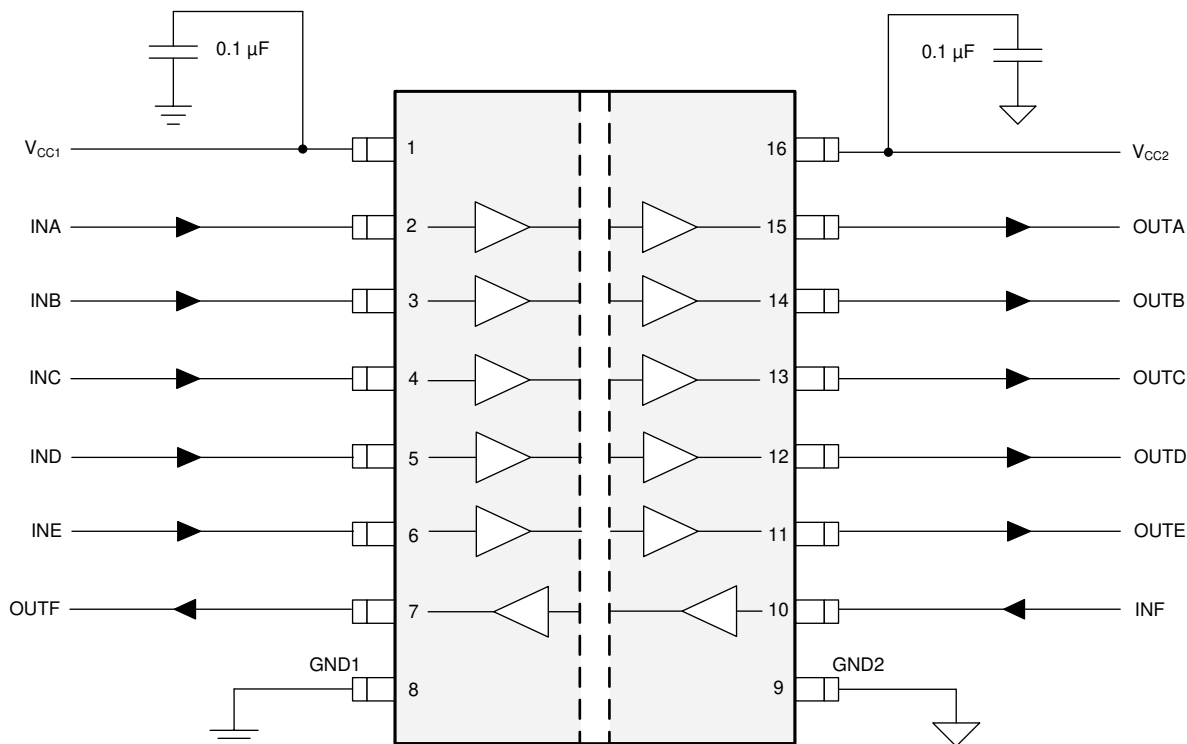
図 8-2. Typical ISO7761-Q1 Circuit Hook-up
