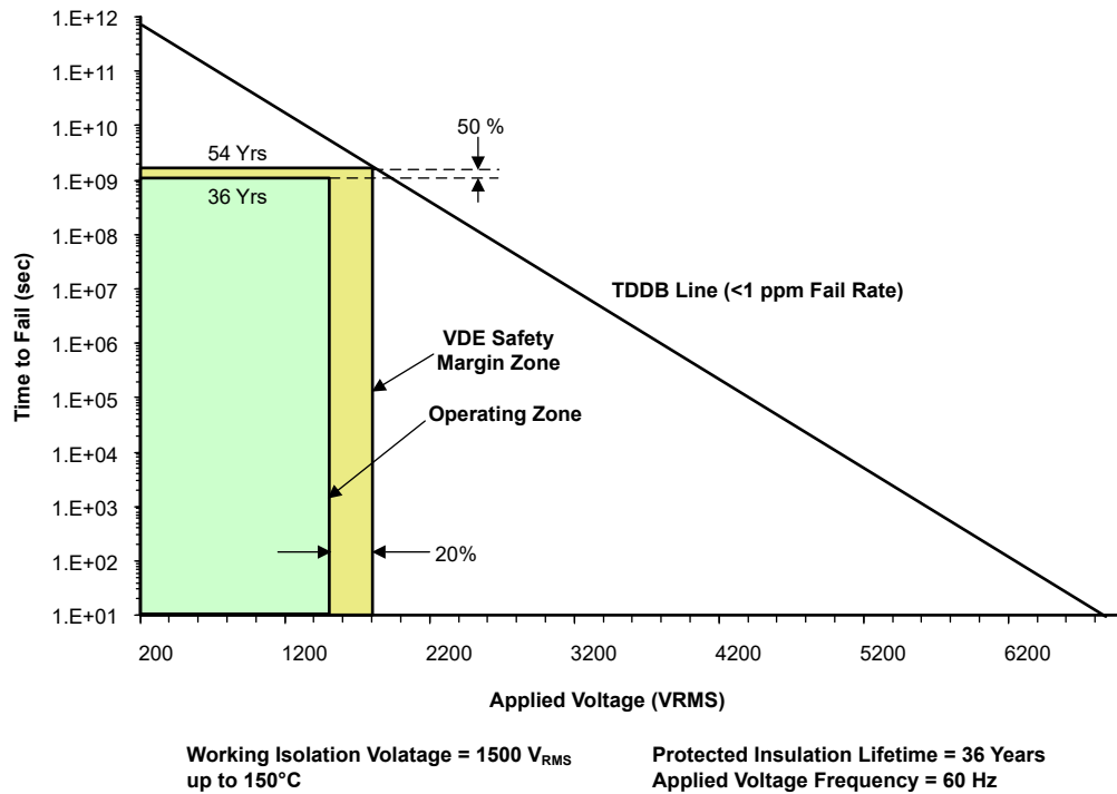
図 8-7. Insulation Lifetime Projection Data
