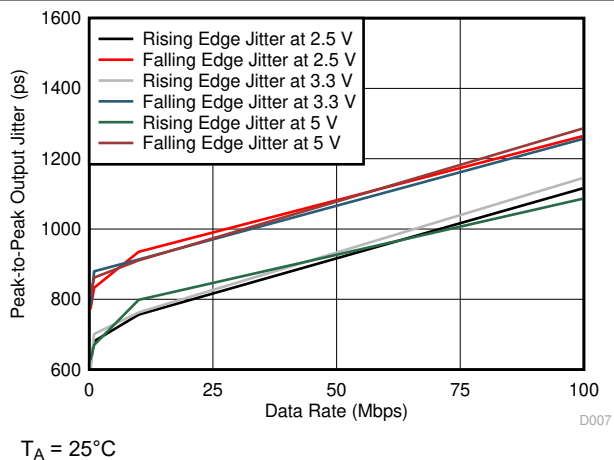
6-17. Peak-to-Peak Output Jitter vs Data Rate
