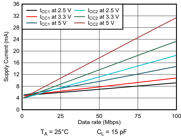
Figure 6-7. ISO7761-Q1 Supply Current vs Data Rate (With 15-pF Load)
