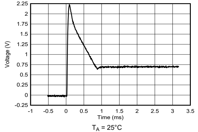
Figure 5-8. Output vs. Settling Time to Step V_{DD}
