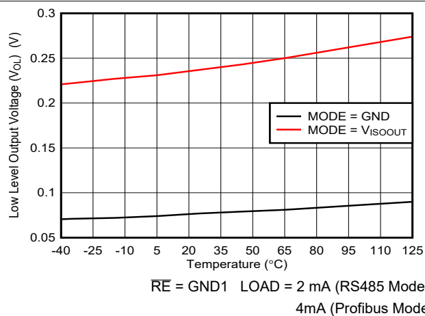
8-20. ISOW1412 Receiver Buffer Low Level output voltage vs. Temperature - RS485 & Profibus Mode
