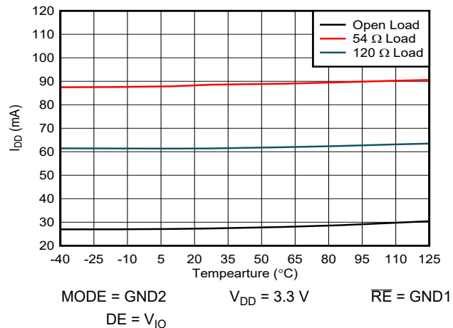
FIG 8-5. ISOW1412 V_{DD} Current vs. Temperature - RS485 Mode
