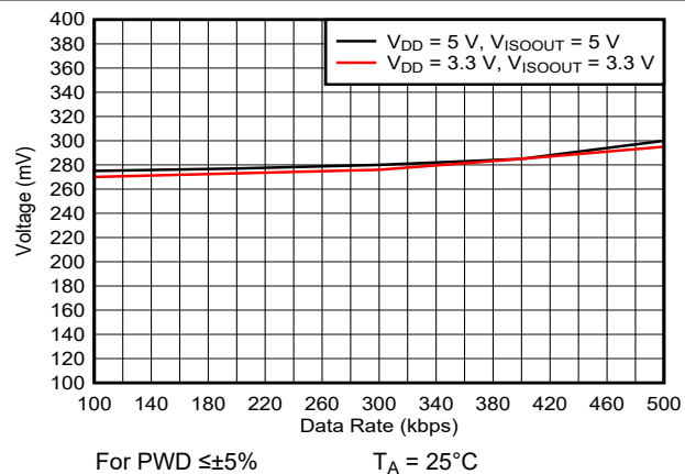
8-21. ISOW1412 Receiver VID vs. Data Rate - RS485 & Profibus Mode
