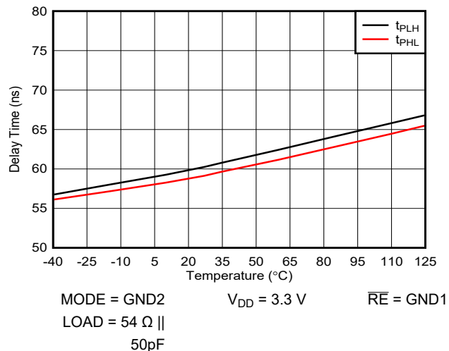
8-9. ISOW1412 Receiver Propagation Delay vs. Temperature - RS485 Mode
