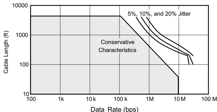
FIG 11-4. Cable length vs Data rate characteristics
