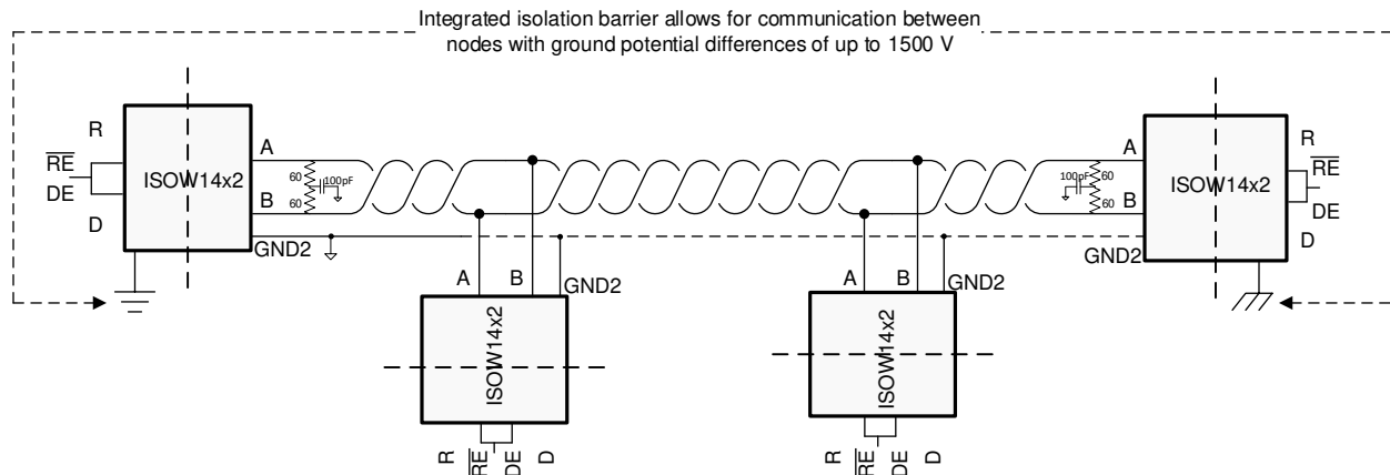
FIG 11-2. Typical RS-485 Network With Half-Duplex Isolated Transceivers
