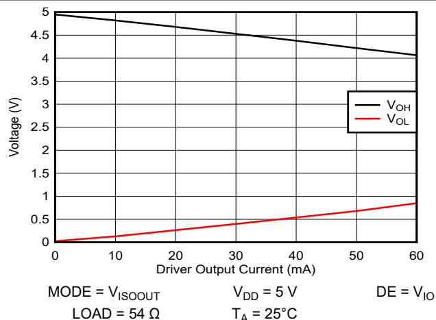
8-16. ISOW1412 Driver output voltage vs. Driver output current - Profibus Mode
