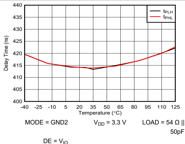
8-7. ISOW1412 Driver Propagation Delay vs. Temperature - RS485 Mode
