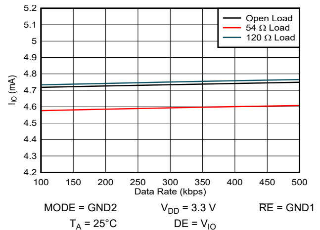
FIG 8-4. ISOW1412 V_{IO} Supply Current vs. Data Rate - RS485 Mode
