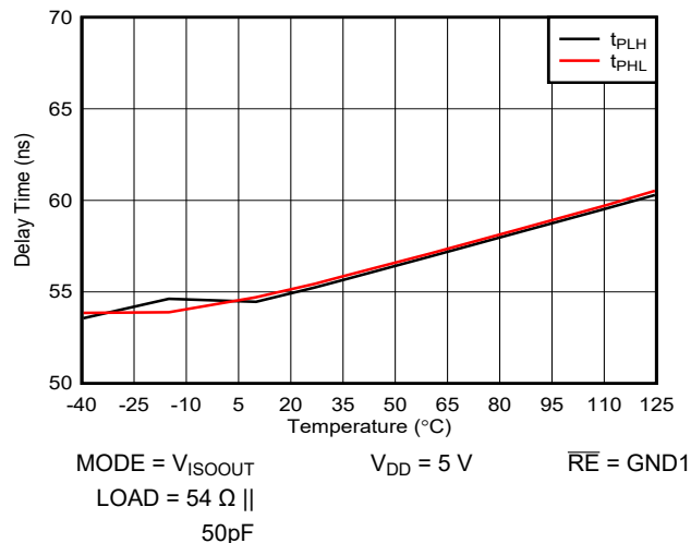
8-10. ISOW1412 Receiver Propagation Delay vs. Temperature - Profibus Mode
