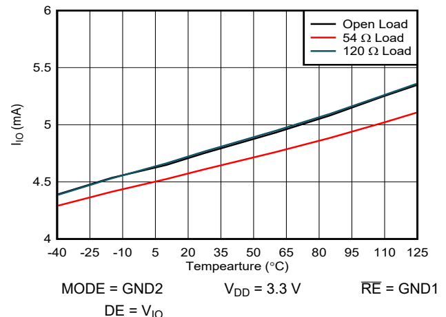
FIG 8-6. ISOW1412 V_{IO} Current vs. Temperature - RS485 Mode
