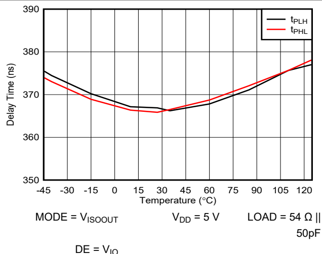
8-8. ISOW1412 Driver Propagation Delay vs. Temperature - Profibus Mode
