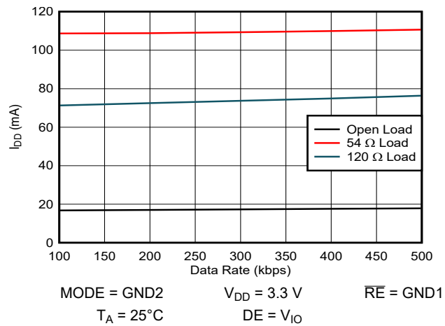
FIG 8-3. ISOW1412 V_{DD} Supply Current vs. Data Rate - RS485 Mode
