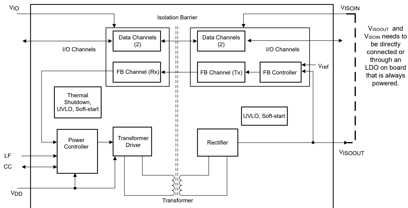
9-1. Block Diagram
