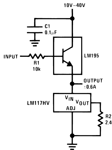
☒ 9-9. Power Follower
