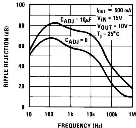
7-8. Ripple Rejection
