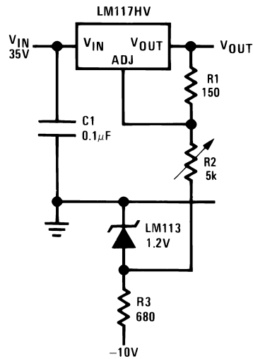
☒ 9-8. 0-V to 30-V Regulator
