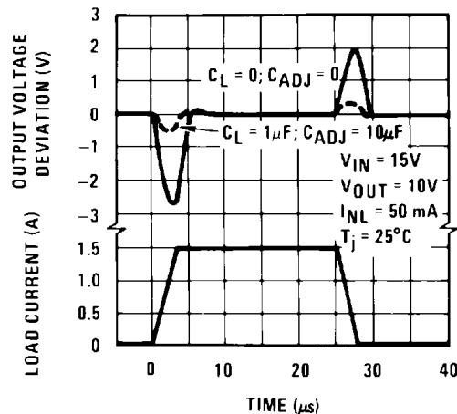
7-12. Load Transient Response
