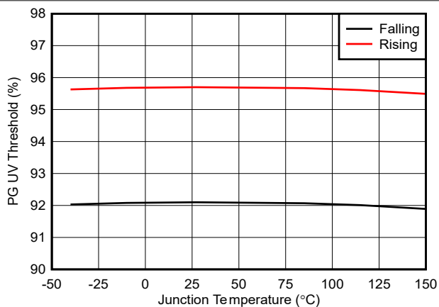
図 7-10. PG UV Thresholds vs Temperature
