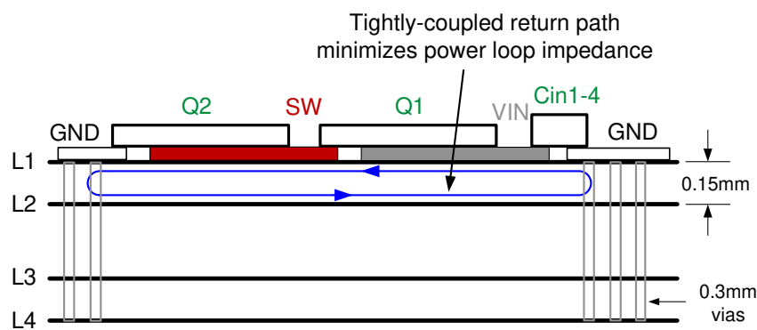
図 9-38. PCB Stack-up Diagram With Low L1-L2 Intra-layer Spacing 1
