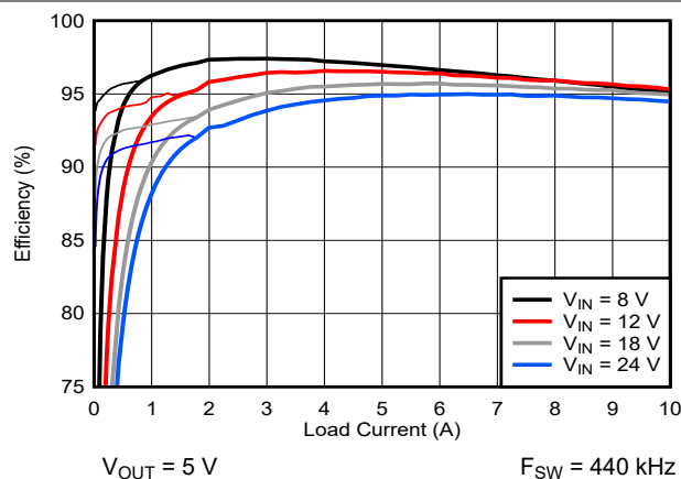
図 7-1. Efficiency vs Load
