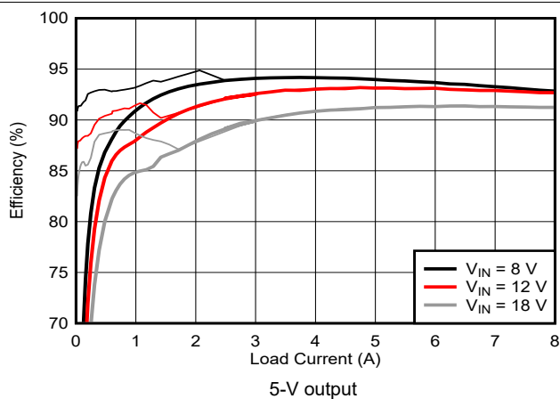
図 9-5. Efficiency vs I_{OUT}
