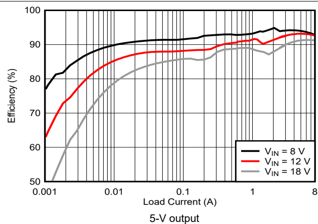
図 9-6. Efficiency vs I_{OUT} , Log Scale
