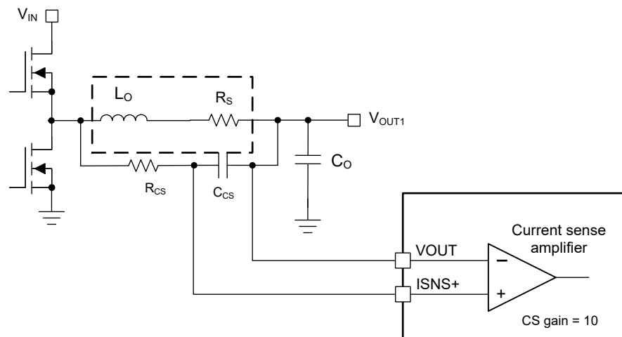
図 8-5. Inductor DCR Current Sensing Implementation
