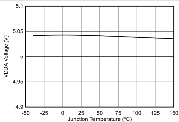
図 7-14. VDDA Regulation Voltage vs Temperature
