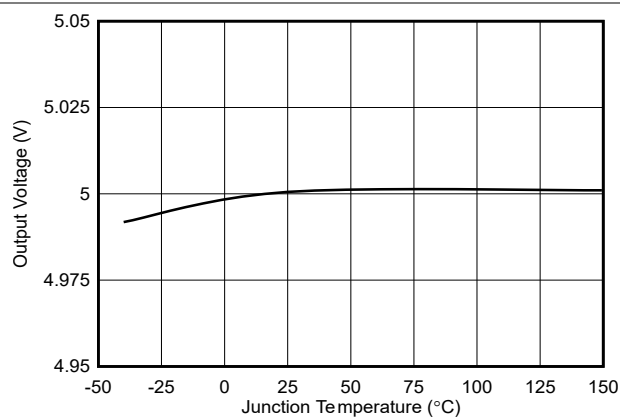
図 7-7. Fixed 5-V Output Voltage vs Temperature
