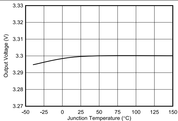
図 7-6. Fixed 3.3-V Output Voltage vs Temperature
