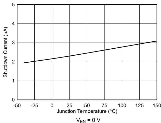
図 7-3. Shutdown Current vs Temperature
