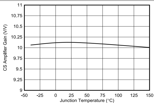
図 7-18. Current Sense (CS) Amplifier Gain vs Temperature
