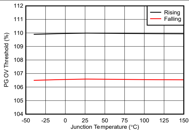
図 7-9. PG OV Thresholds vs Temperature
