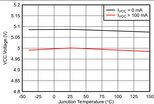
図 7-11. VCC Regulation Voltage vs Temperature
