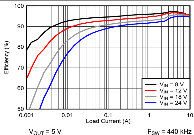
図 7-2. Efficiency vs Load, Log Scale
