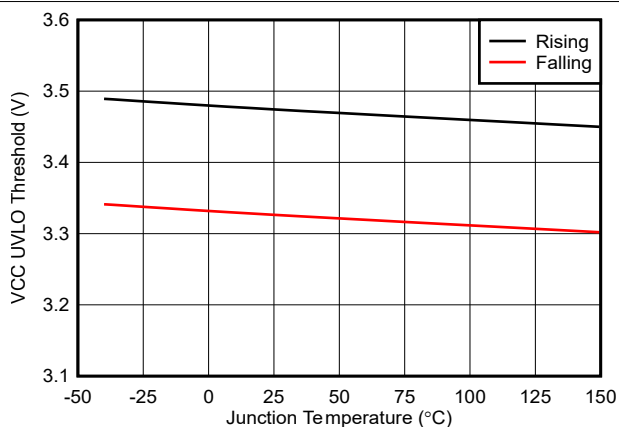
図 7-12. VCC UVLO Thresholds vs Temperature
