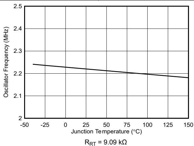
FIG 7-21. Switching Frequency vs Temperature
