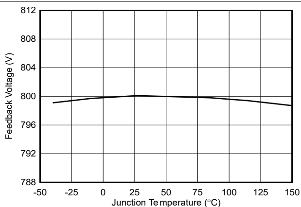
図 7-8. Feedback Voltage vs Temperature
