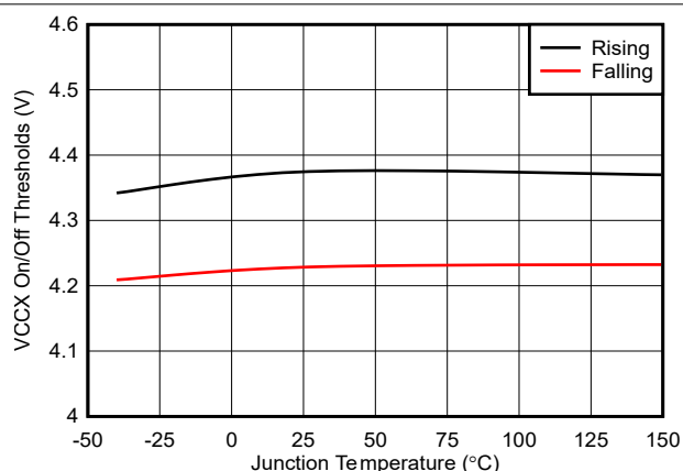
図 7-16. VCCX On, Off Thresholds vs Temperature
