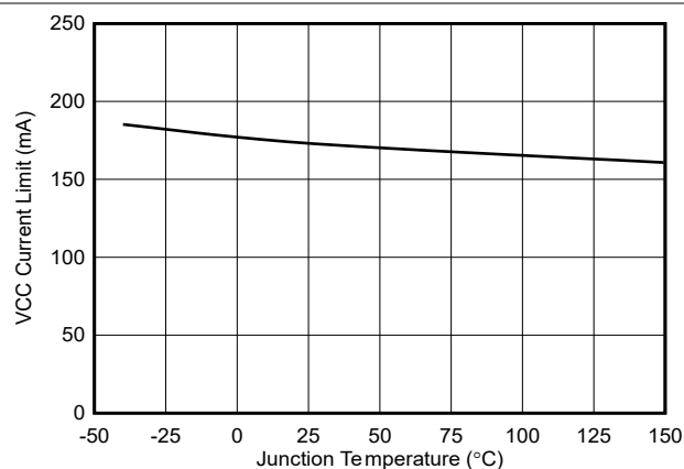
図 7-13. VCC Current Limit vs Temperature
