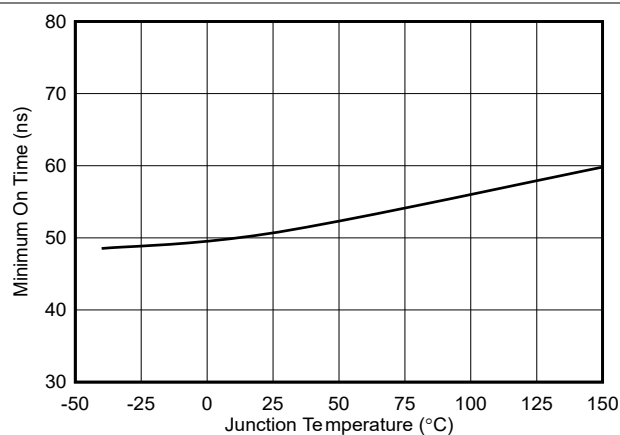
FIG 7-19. Minimum On Time (HO) vs Temperature
