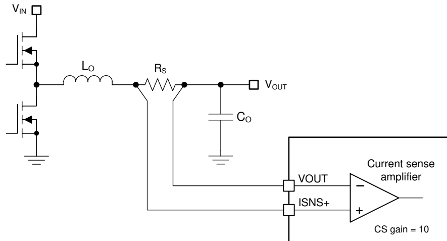
図 8-4. Shunt Current Sensing Implementation
