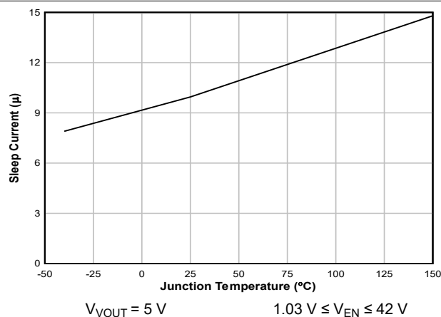
図 7-5. Sleep2 Current vs Temperature
