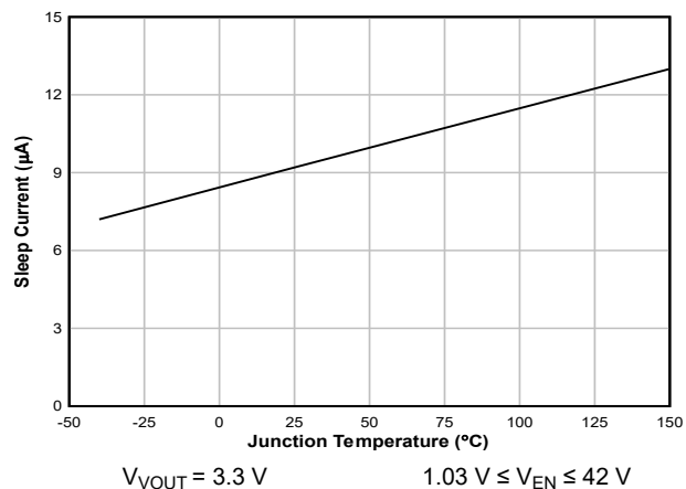
図 7-4. Sleep1 Current vs Temperature
