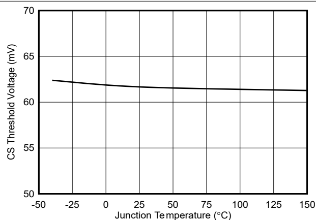
図 7-17. Current Sense (CS) Threshold vs Temperature
