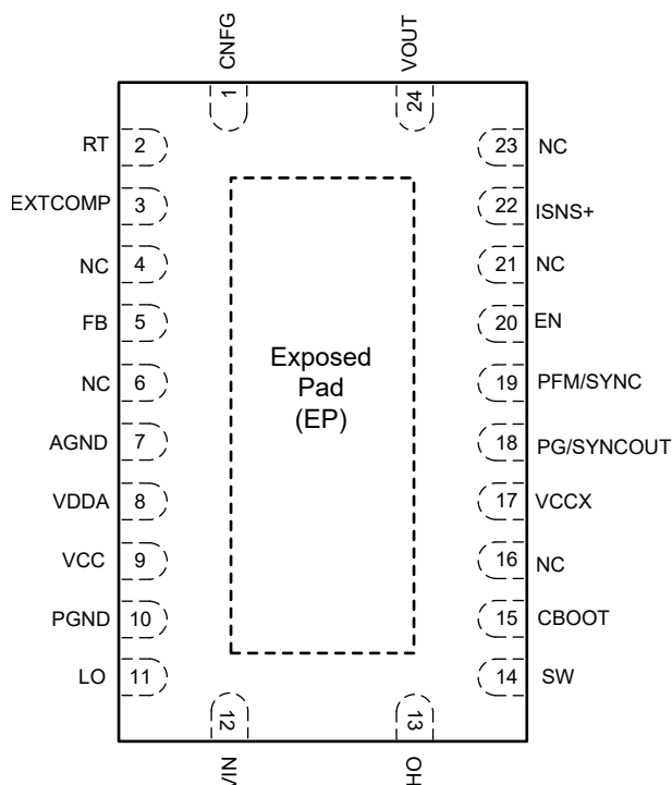
図 6-2. 24-Pin VQFN RGY Package With Wettable Flanks, LM25148BQRGYRQ1 (Top View)
