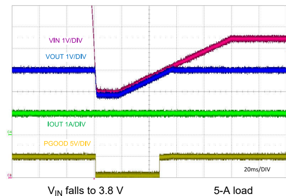
図 9-10. Cold-Crank Response to V_{IN} = 3.8 V
