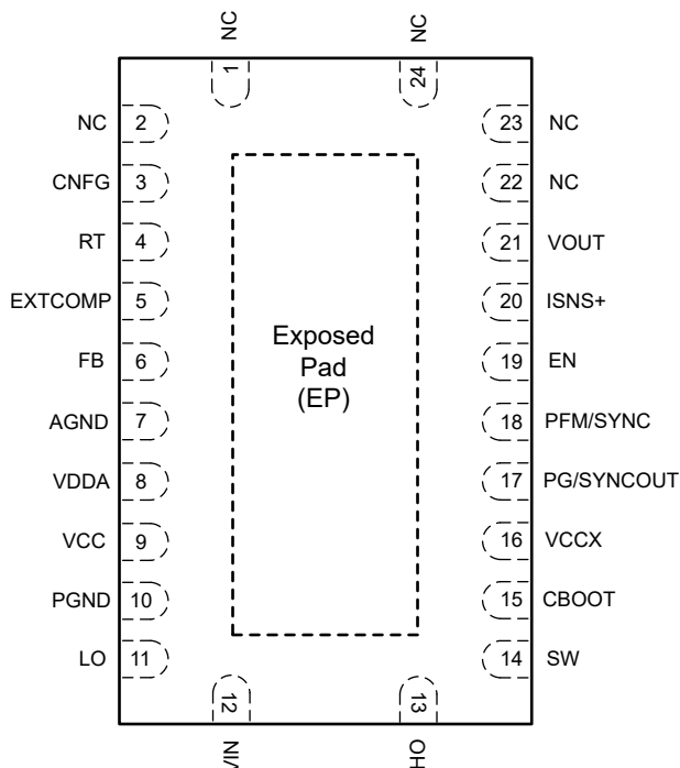
図 6-1. 24-Pin VQFN RGY Package With Wettable Flanks, LM25148QRGYRQ1 (Top View)
