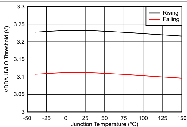
図 7-15. VDDA UVLO Thresholds vs Temperature
