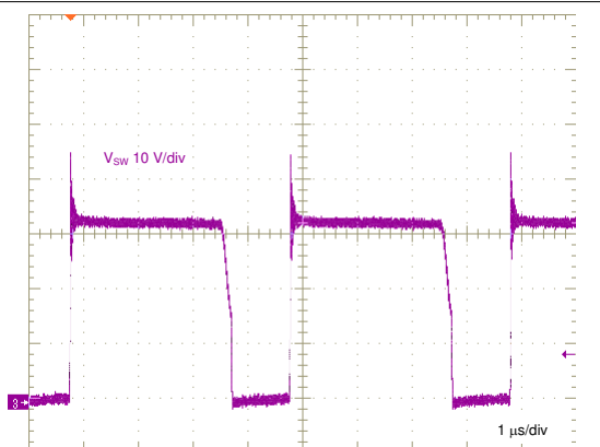
8-23. Switch Voltage, No Load
