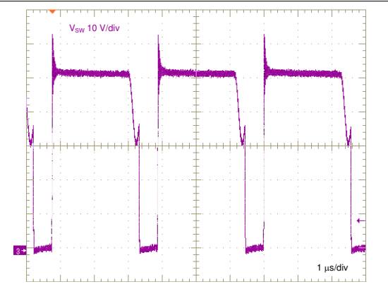
8-26. Switch Voltage, Full Load
