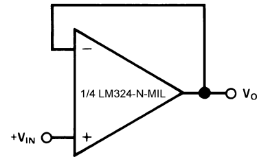
Figure 23. Voltage Follower
