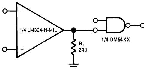
Figure 22. Driving TTL
