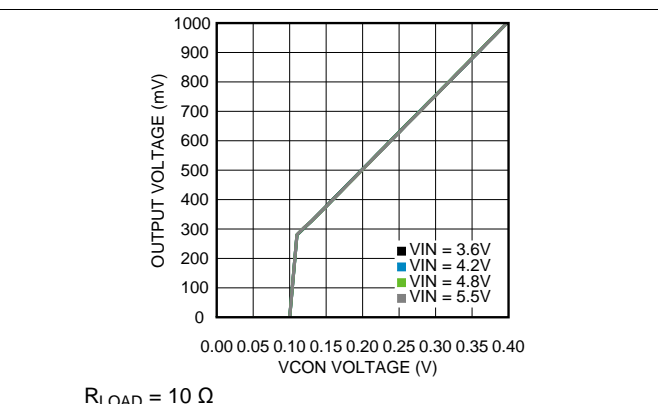
Figure 22. Low VCON Voltage vs Output Voltage
