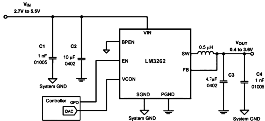
Figure 29. Simplified LM3262 RF Evaluation Board Schematic
