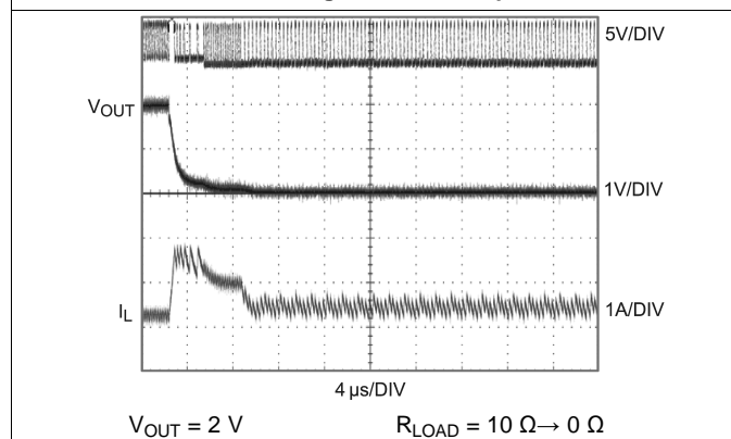
Figure 21. Timed Current Limit
