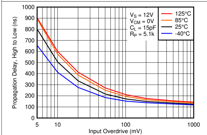
7-27. High to Low Propagation Delay vs. Input Overdrive Voltage, 12V
