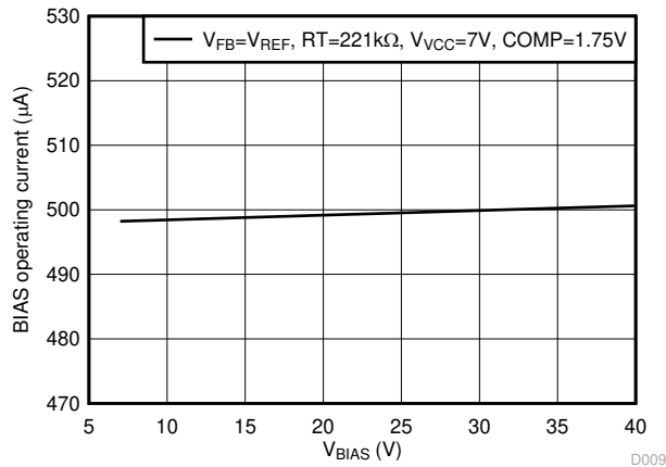
7-9. I_{OPERATING(BIAS)} Including RT Current vs V_{BIAS}
