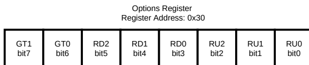
Figure 22. Options Register Internal Hex Address: 0x30
