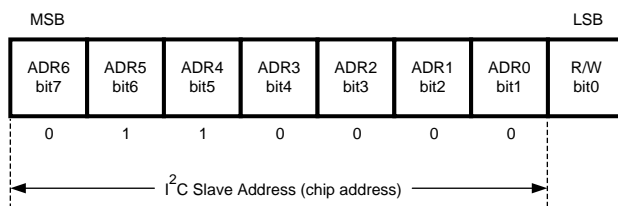
Figure 44. Device Address
