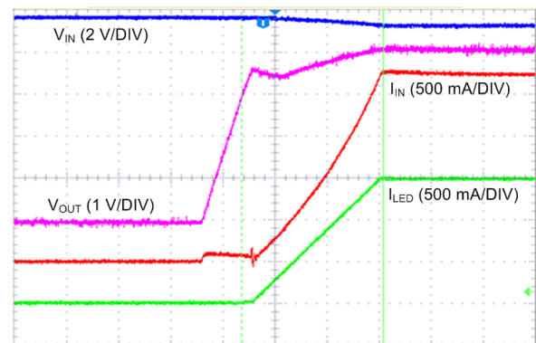
Time (400 μs/DIV) Reg 0x01 = 0x24
