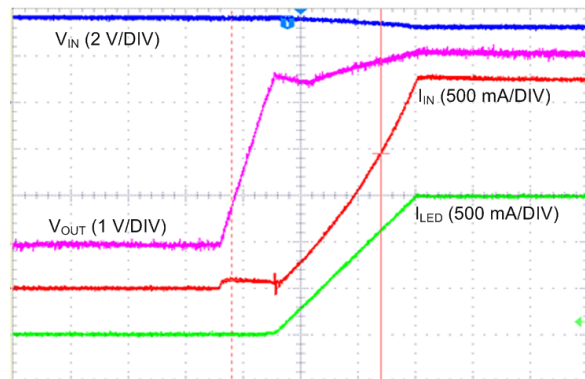
Time (400 μs/DIV) Reg 0x01 = 0x2C
