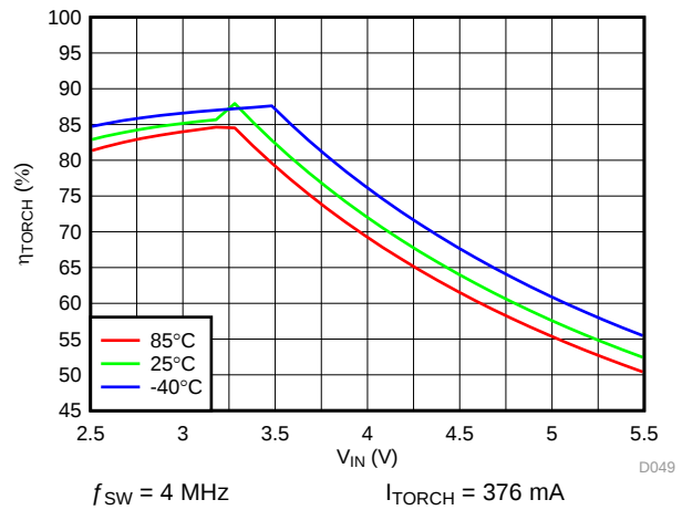
FIG 59. LED Torch Efficiency vs Input Voltage
