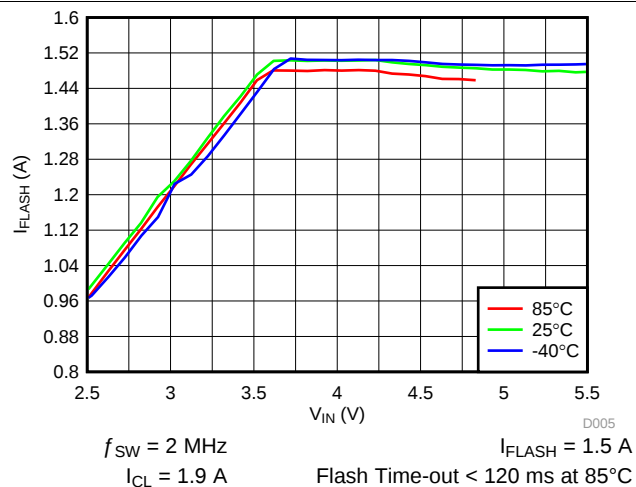
图 6. LED Flash Current vs Input Voltage
