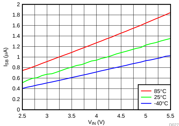
FIG 26. LED Off Current vs Input Voltage
