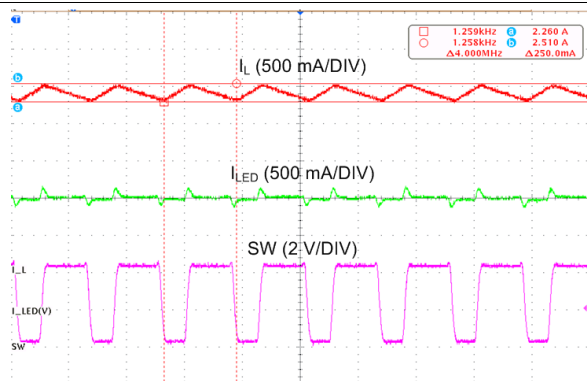
FIG 77. Pass mode Level Triggered Flash
