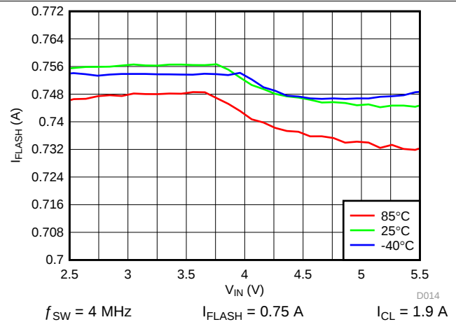
Figure 15. LED Flash Current vs Input Voltage
