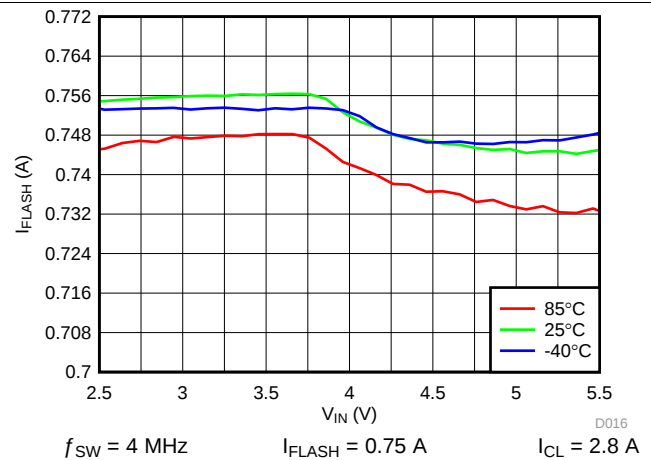
Figure 17. LED Flash Current vs Input Voltage
