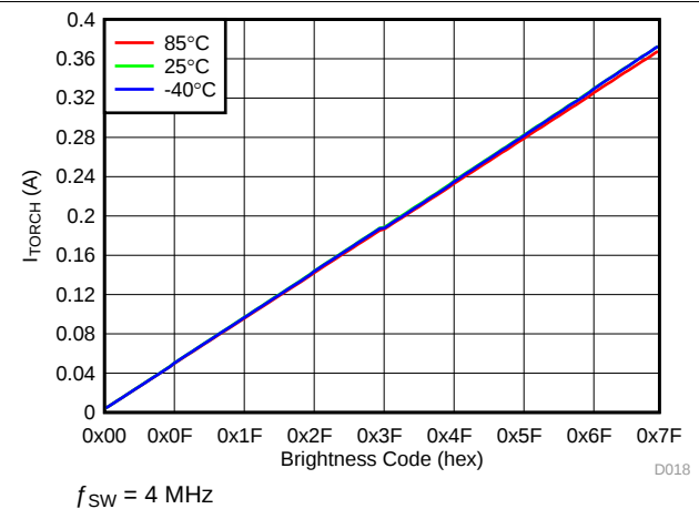
Figure 19. LED Torch Current vs Brightness Code
