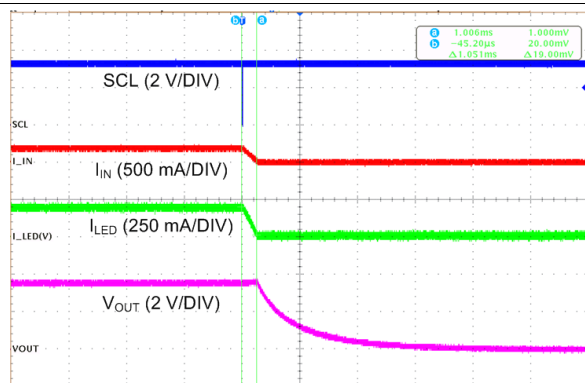
Time (4 ms/DIV)
