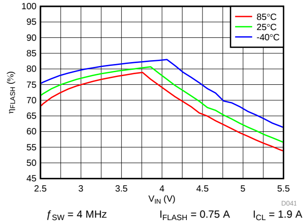
FIG 51. LED Flash Efficiency vs Input Voltage
