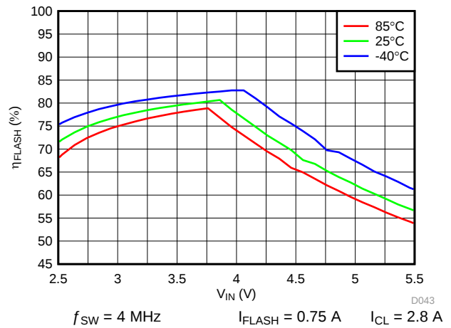
FIG 53. LED Flash Efficiency vs Input Voltage
