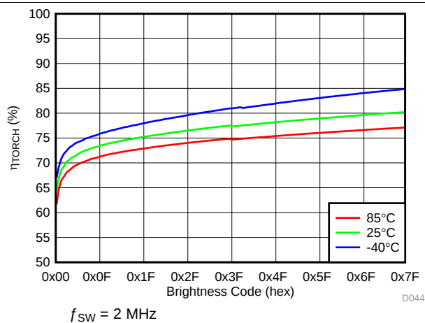
FIG 54. LED Torch Efficiency vs Brightness Code
