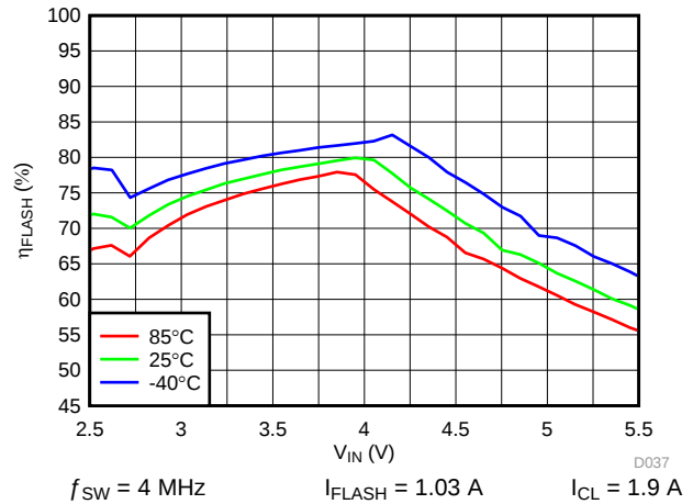
FIG 47. LED Flash Efficiency vs Input Voltage
