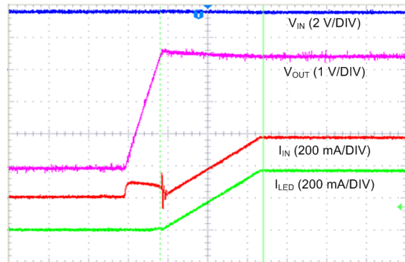
Time (400 μs/DIV) Reg 0x01 = 0x26
