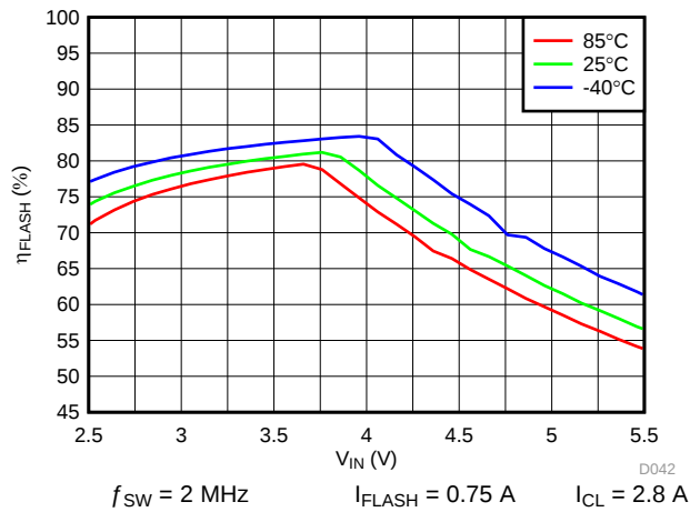
FIG 52. LED Flash Efficiency vs Input Voltage
