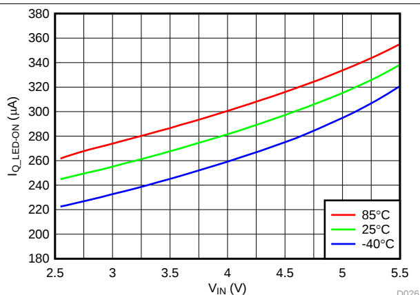
FIG 27. LED On Current vs Input Voltage
