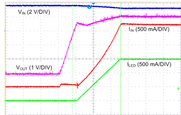
Time (400 μs/DIV) Reg 0x01 = 0x27
