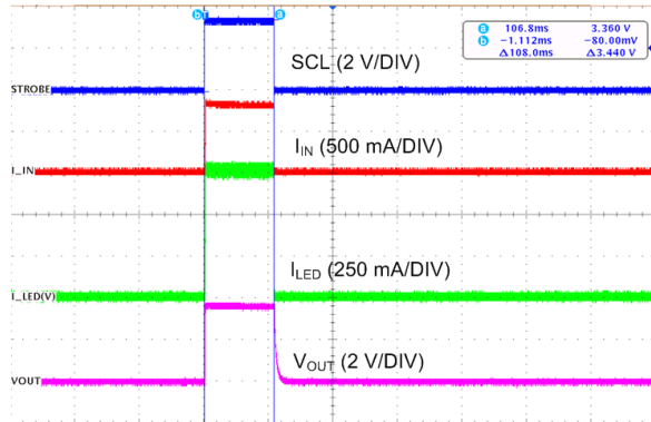
Time (100 ms/DIV) STROBE Enabled (Reg 0x01 bit[2] = 1) Level Triggered (Reg 0x01 bit[3] = 0) Strobe pulse = 100 ms
