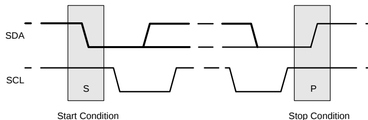
✎ 34. Start and Stop Conditions
