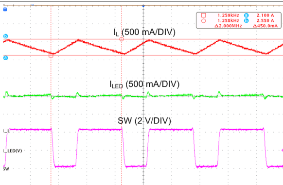
FIG 76. Pass mode Edge Triggered Flash
