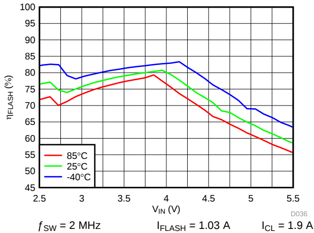
FIG 46. LED Flash Efficiency vs Input Voltage
