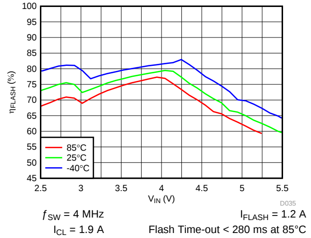
FIG 45. LED Flash Efficiency vs Input Voltage
