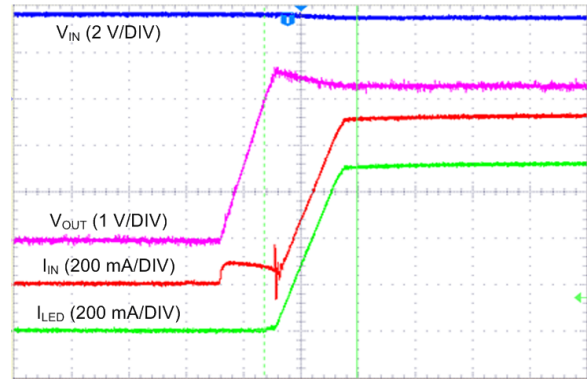
FIG 75. Pass Mode I 2 C Flash
