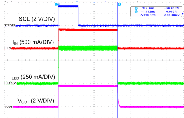
Time (100 ms/DIV) STROBE Enabled (Reg 0x01 bit[2] = 1) Edge Triggered (Reg 0x01 bit[3] = 1) Flash Time-out = 320 ms
