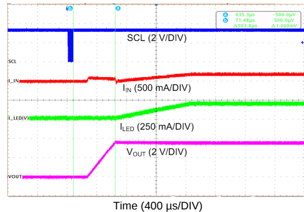
Time (400 \mu\text{s} /DIV) Mode bits (Reg 0x01 bit[1:0]) = 10 (Torch Mode)
