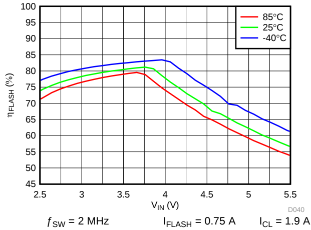
FIG 50. LED Flash Efficiency vs Input Voltage
