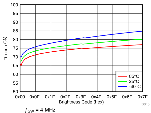
FIG 55. LED Torch Efficiency vs Brightness Code
