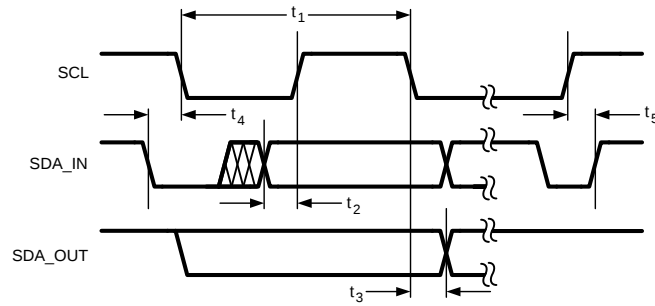
図 1. I²C-Compatible Interface Specifications
