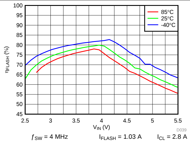
FIG 49. LED Flash Efficiency vs Input Voltage
