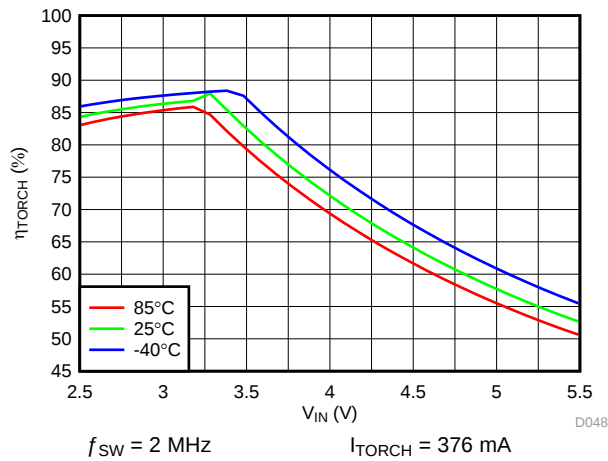
FIG 58. LED Torch Efficiency vs Input Voltage
