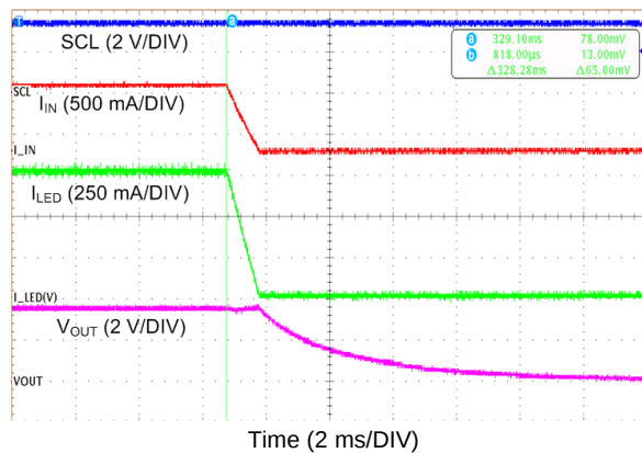
Time (2 ms/DIV)
