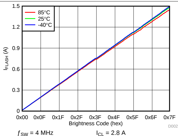
图 3. LED Flash Current vs Brightness Code
