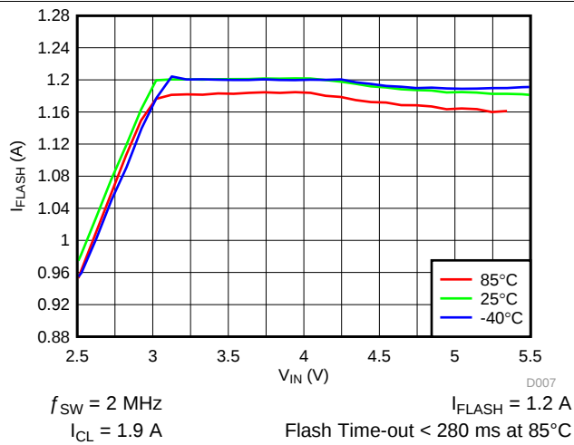
Figure 8. LED Flash Current vs Input Voltage
