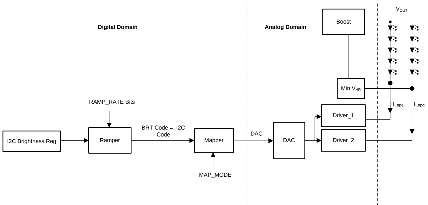
FIG 34. I 2 C Only Brightness Control
