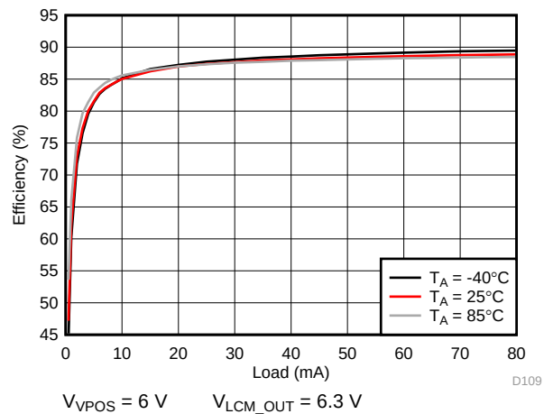
123. VPOS Efficiency
