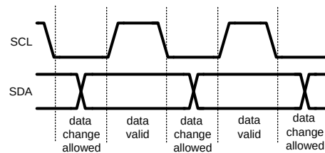
FIG 42. Data Validity
