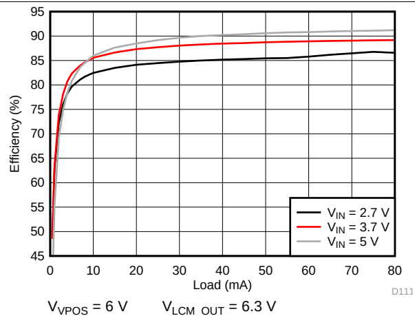
125. VPOS Efficiency
