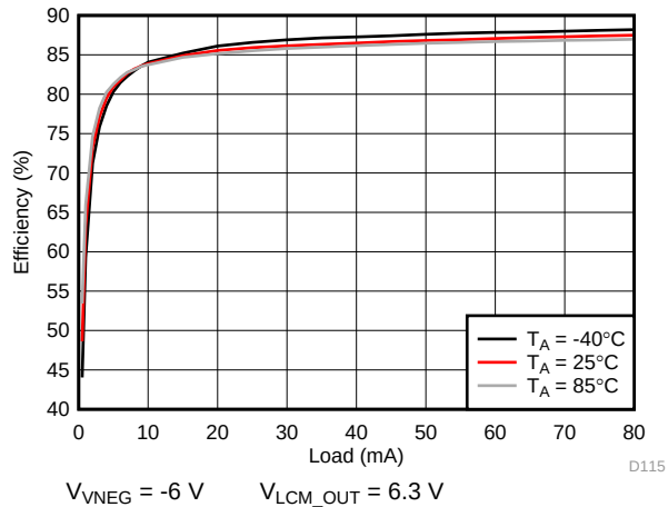
Figure 129. VNEG Efficiency
