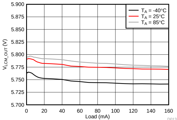
FIG 14. Backlight Regulated Headroom Voltage
