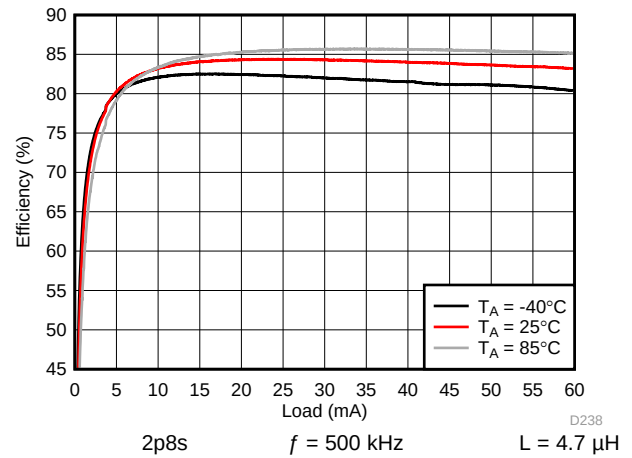
图 106. Backlight System Efficiency
