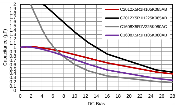
FIG 68. DC Bias Derating for 0805 Case Size and 0603 Case Size 35-V and 50-V Ceramic Capacitors
