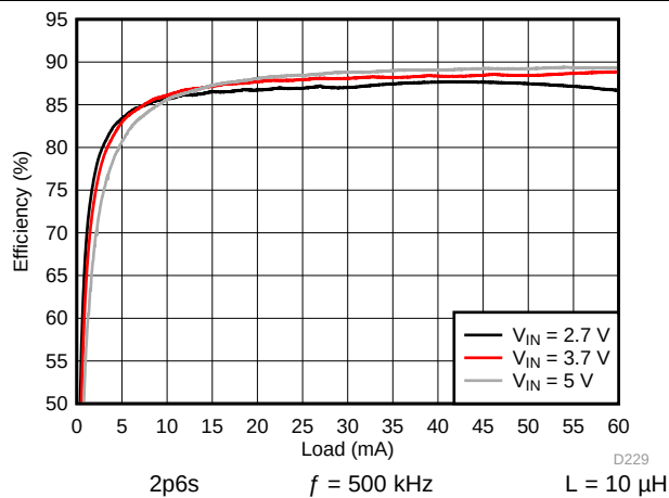
图 97. Backlight Boost Efficiency
