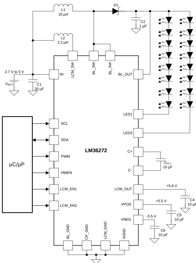
67. LM36272 Typical Application
