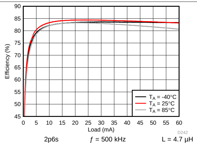
图 110. Backlight System Efficiency
