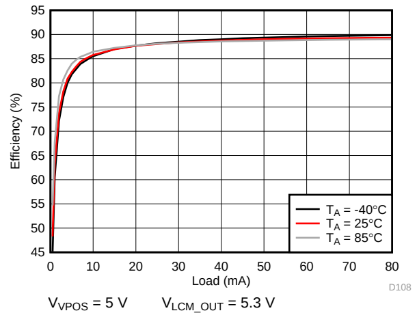
122. VPOS Efficiency
