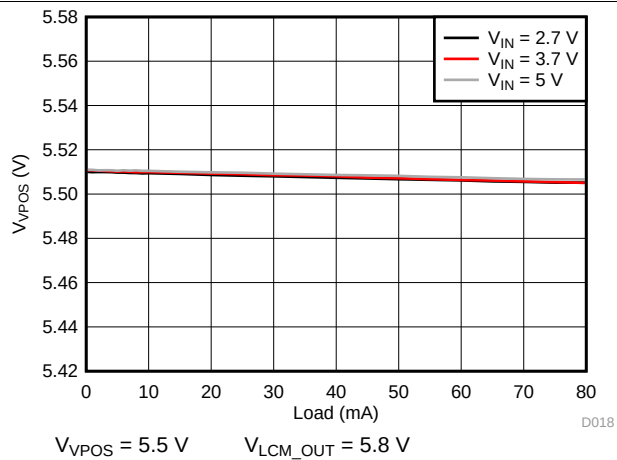
Figure 21. V_{VPOS} Load Regulation
