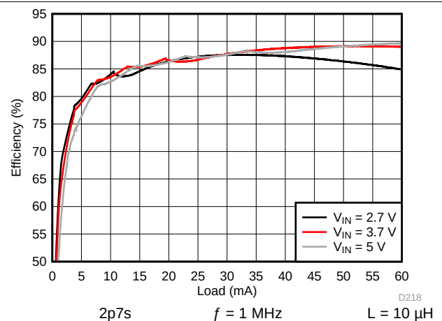
图 86. Backlight System Efficiency
