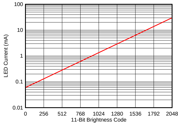
FIG 33. LED Current vs Brightness Code (Exponential Mapping)
