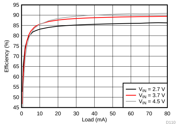
122. VPOS Efficiency
