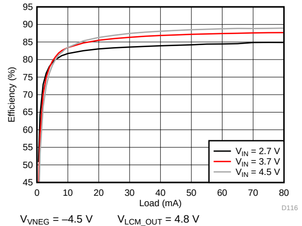
Figure 130. VNEG Efficiency
