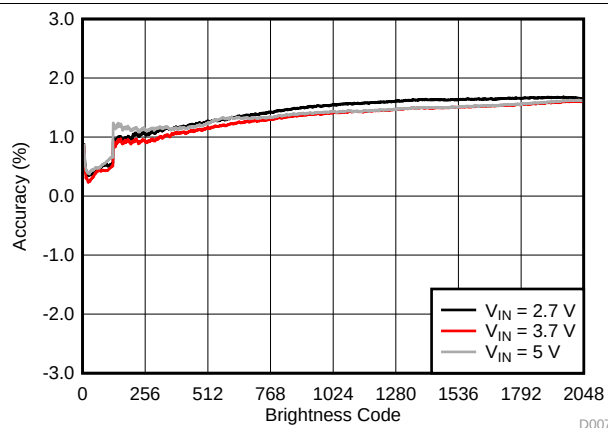
図 8. Backlight LED Current Accuracy
