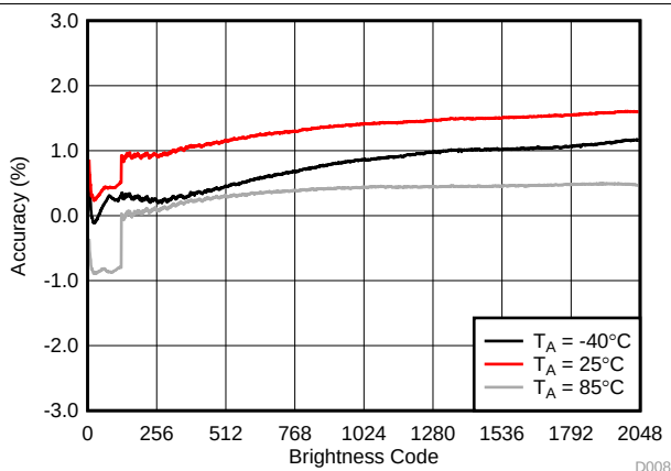
図 9. Backlight LED Current Accuracy
