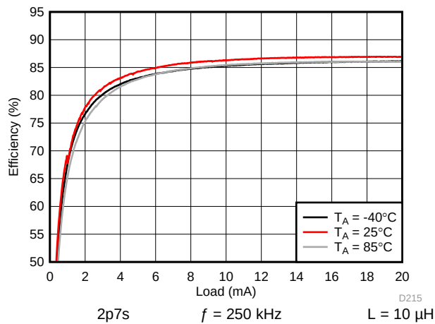
图 83. Backlight Boost Efficiency
