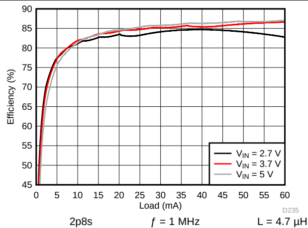
图 103. Backlight Boost Efficiency
