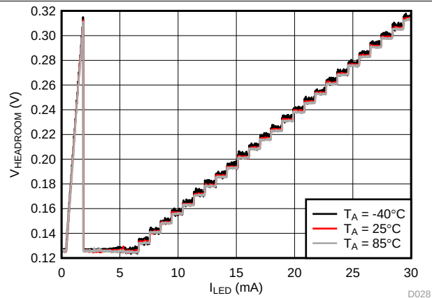
FIG 14. Backlight Regulated Headroom Voltage
