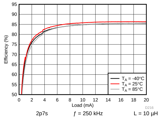
图 84. Backlight System Efficiency
