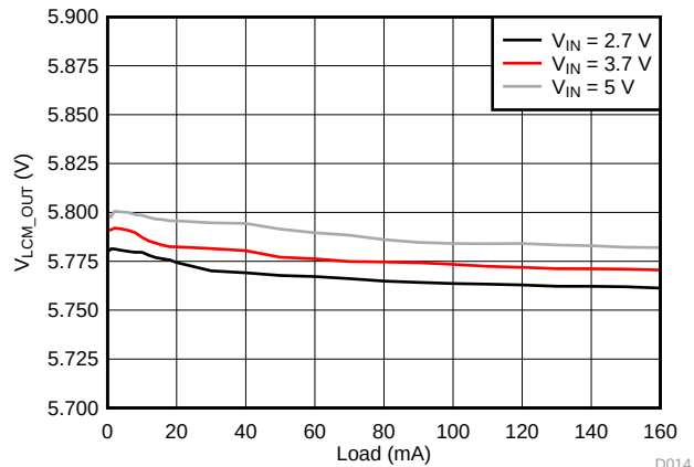
FIG 15. V_{LCM\_OUT} Load Regulation
