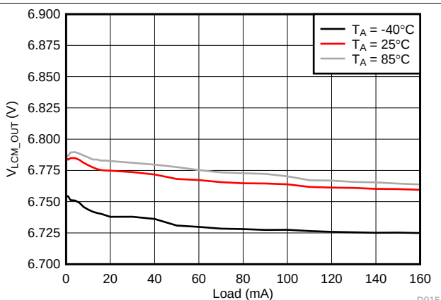
FIG 16. V_{LCM\_OUT} Load Regulation
