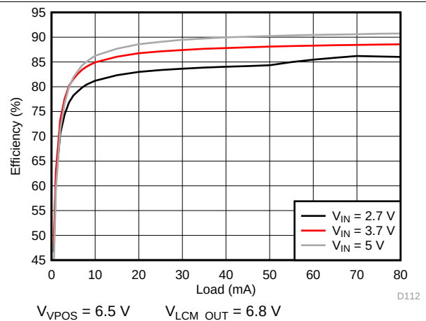
126. VPOS Efficiency
