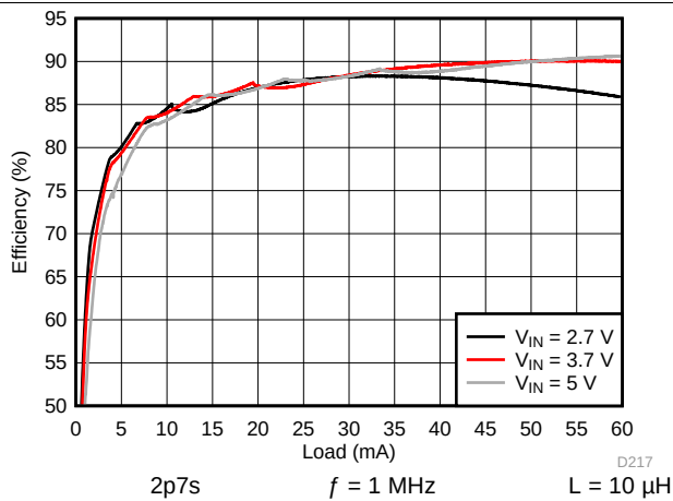
图 85. Backlight Boost Efficiency
