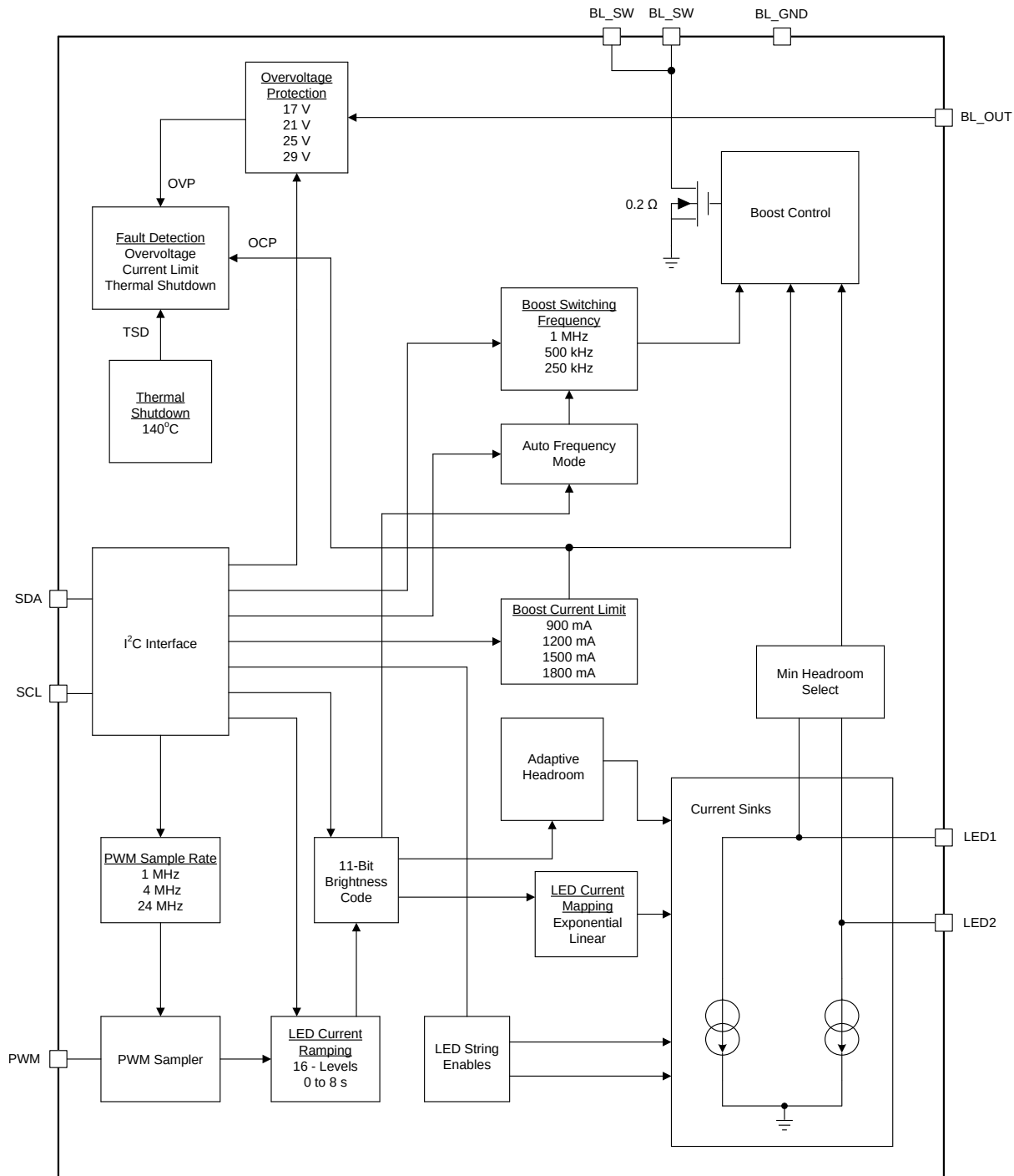
FIG 30. Backlight Block Diagram
