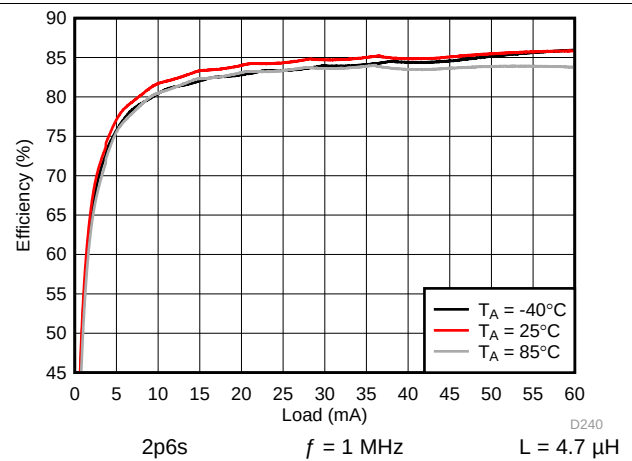
图 108. Backlight System Efficiency
