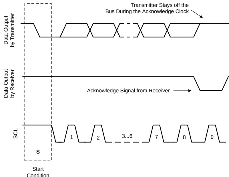
FIG 43. Acknowledge Signal
