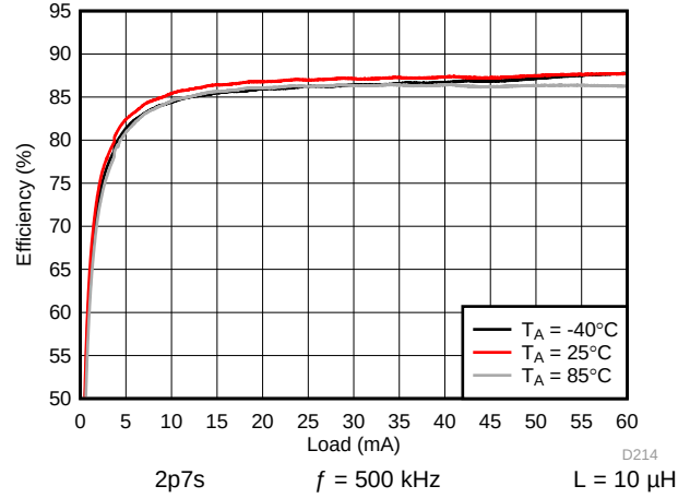
图 82. Backlight System Efficiency
