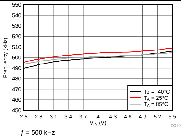
図 11. Backlight Boost Frequency
