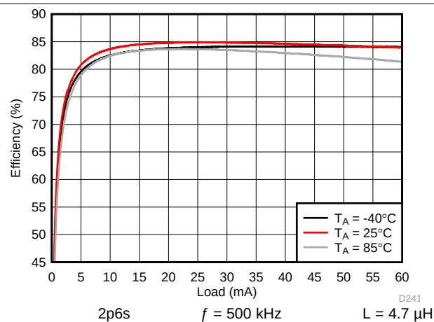
图 109. Backlight Boost Efficiency
