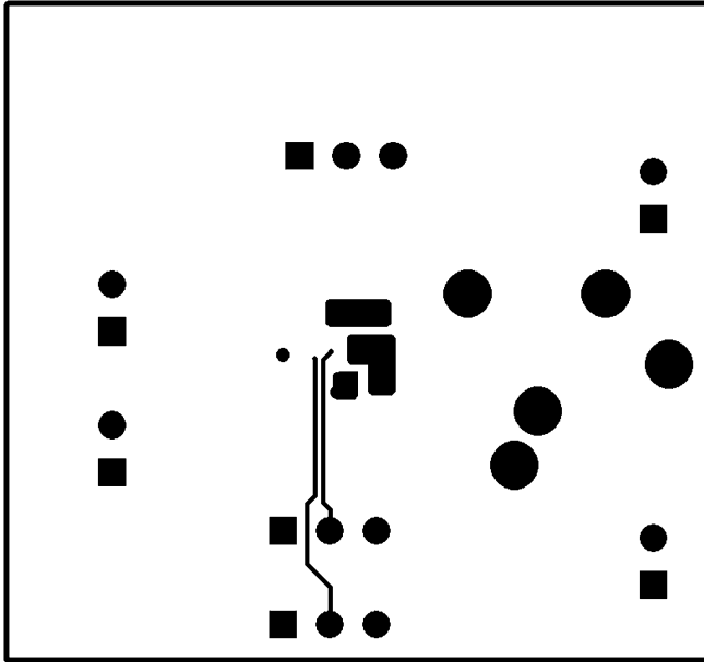
Figure 42. Bottom Layer
