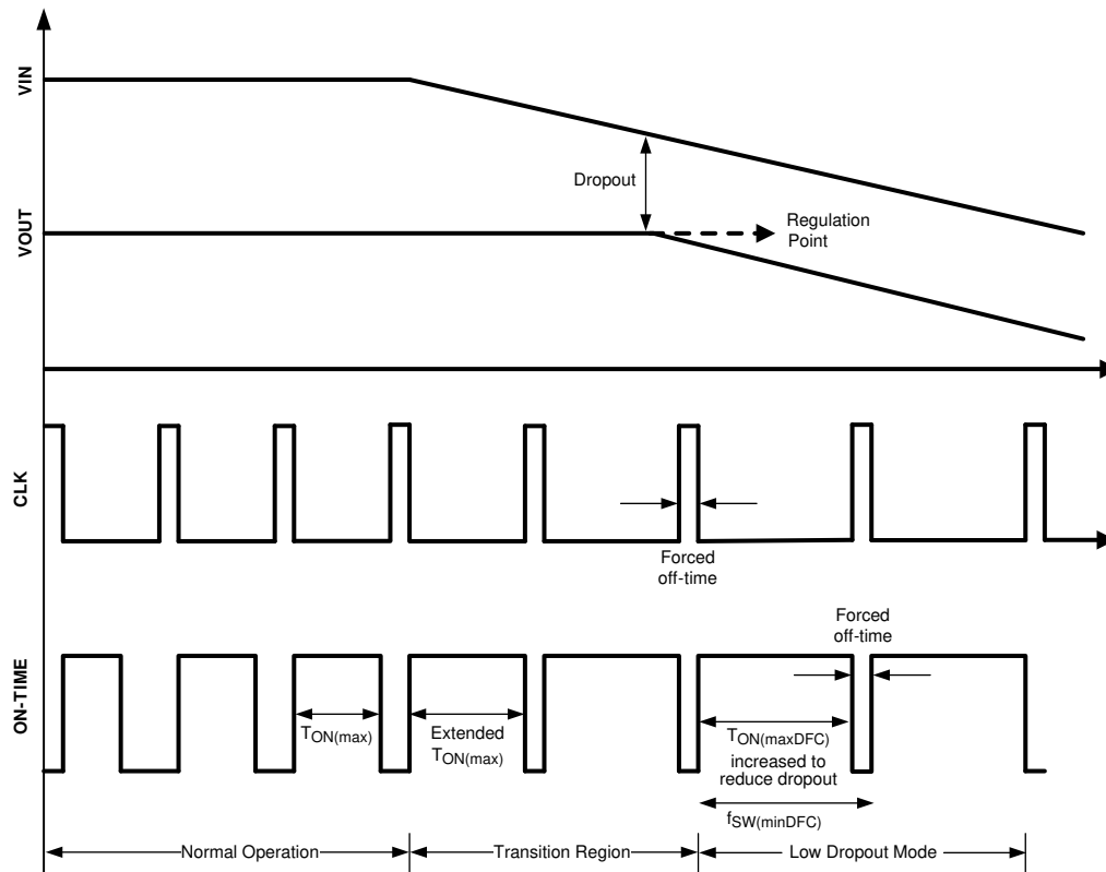
✎ 7-4. Dropout Voltage Reduction using Dynamic Frequency Control
