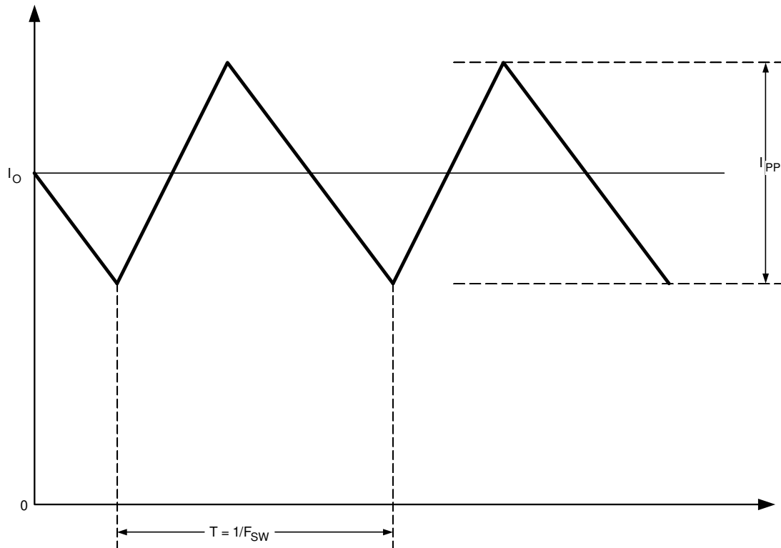
FIG 8-2. Inductor Current
