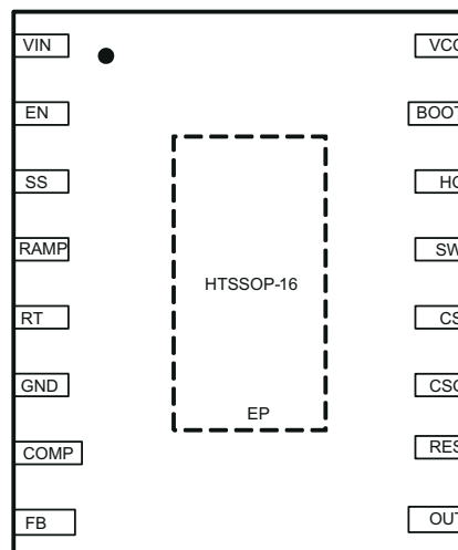
図 5-2. 16-Pin PWP Package (Restart Version) (Top View)
