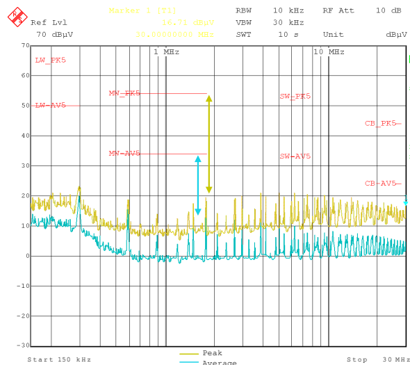
7-14. No-Load Switching
