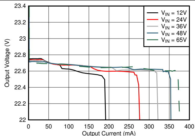
図 41. Load Regulation (Linear Scale)
