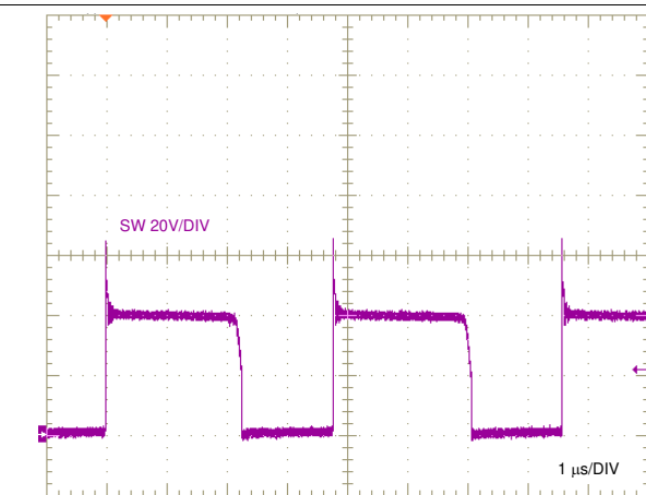
図 45. SW Node Voltage, Full Load
