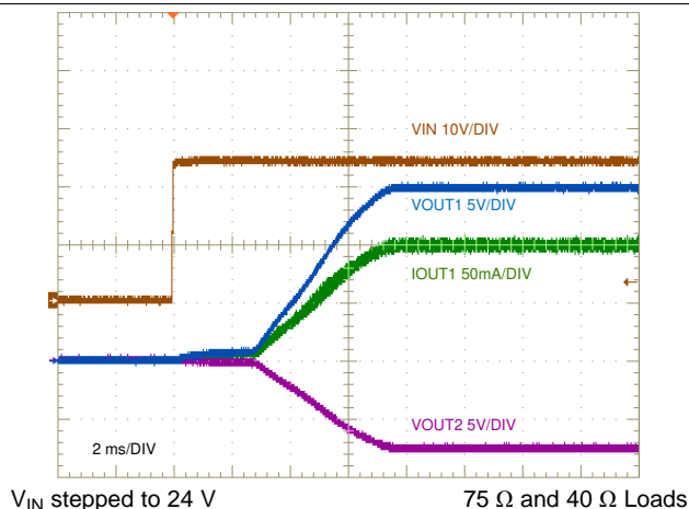
図 43. Start-Up Characteristic
