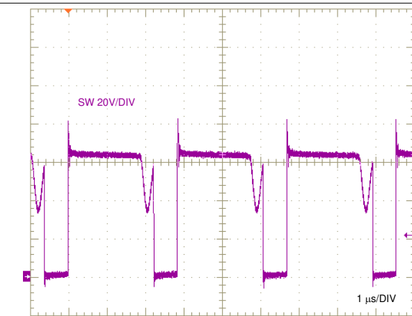
図 46. SW Node Voltage, Full Load
