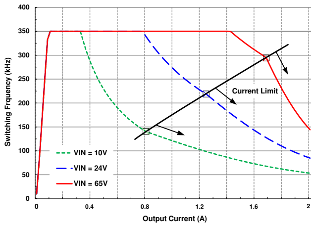
图 28. Switching Frequency Over Load and Line
