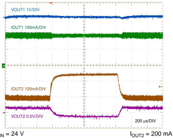
図 50. Output 2 Load Transient, 50 mA to 200 mA
