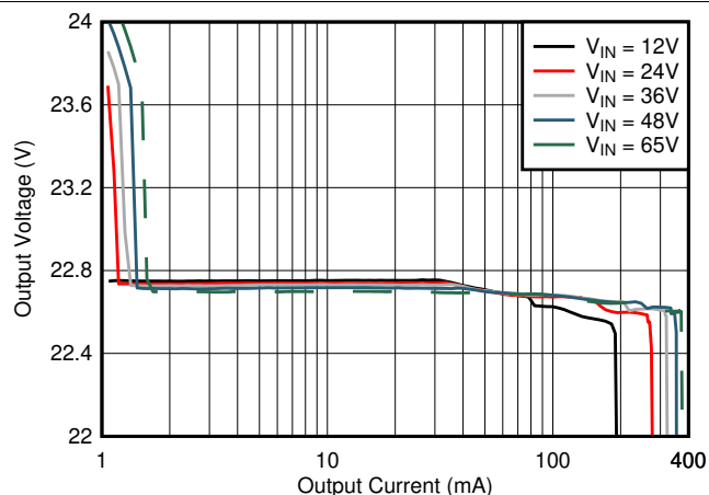
図 42. Load Regulation (Log Scale)
