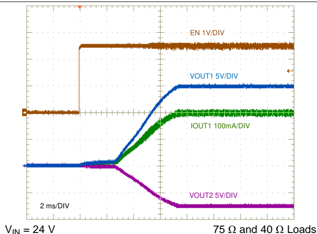
図 44. ENABLE ON Characteristic
