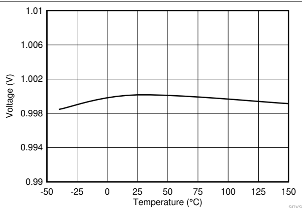
7-3. Feedback Voltage
