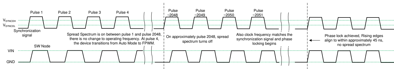
✎ 8-4. Synchronization Process
