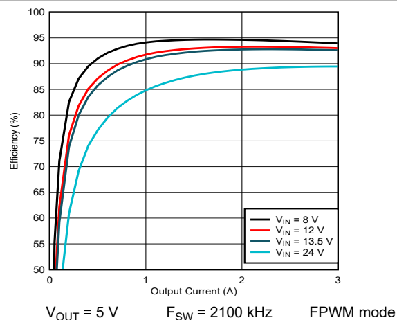
Figure 9-11. LM61430-Q1 Efficiency
