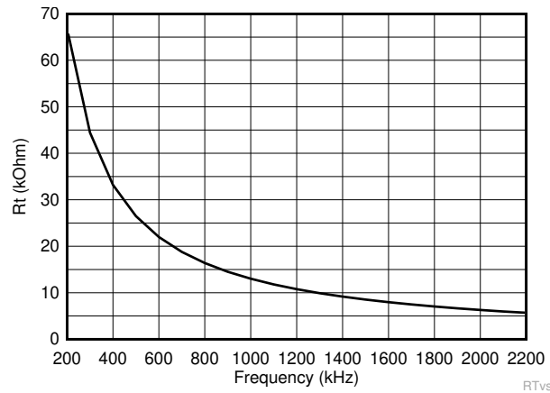
図 8-5. Setting Clock Frequency
