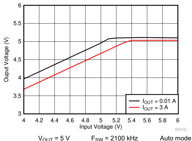
Figure 9-23. LM61430-Q1 Dropout Curve
