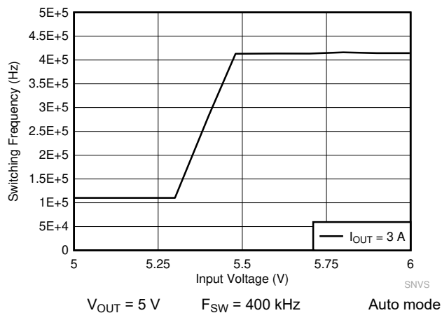
Figure 9-26. LM61430-Q1 Frequency Dropout Curve
