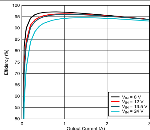
Figure 9-7. LM61430-Q1 Efficiency
