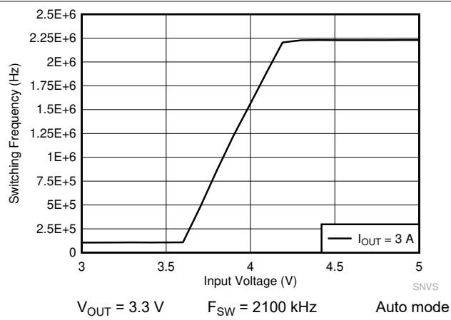
Figure 9-25. LM61430-Q1 Frequency Dropout Curve
