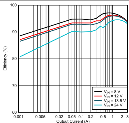
Figure 9-6. LM61430-Q1 Efficiency
