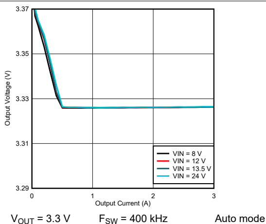
Figure 9-12. LM61430-Q1 Load and Line Regulation
