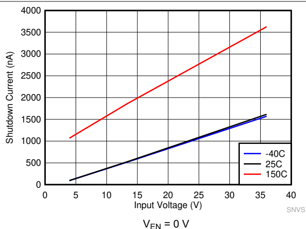
7-2. Shutdown Supply Current
