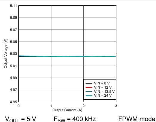
Figure 9-17. LM61430-Q1 Efficiency
