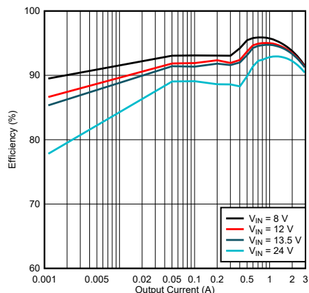
Figure 9-4. LM61430-Q1 Efficiency
