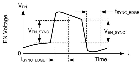
✎ 8-3. Typical SYNC/EN Waveform
