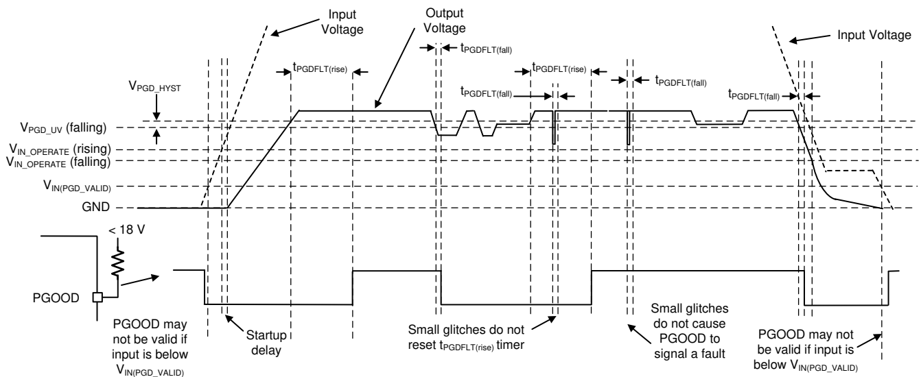
図 8-6. PGOOD Timing Diagram (Excludes OV Events)
