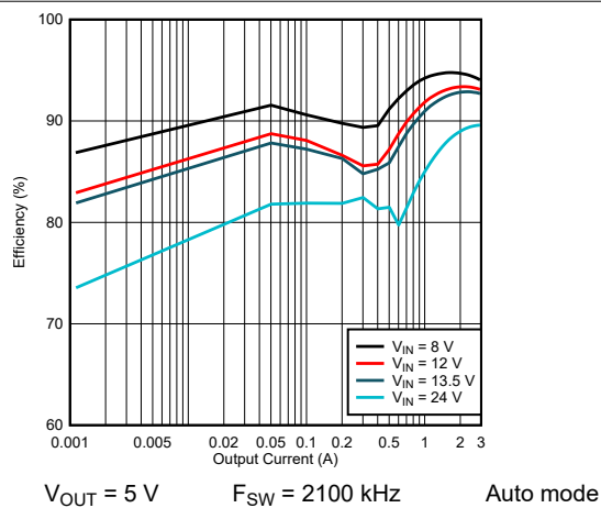
Figure 9-10. LM61430-Q1 Efficiency
