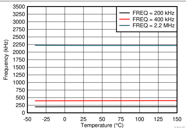
7-4. Switching Frequency Set by RT Resistor
