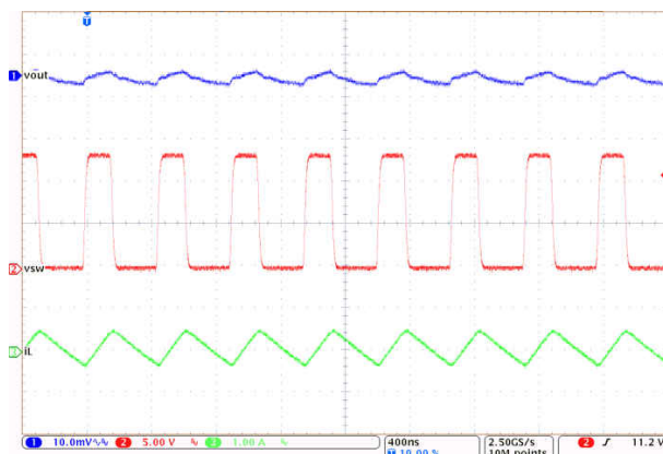
Figure 9-29. LM61430-Q1 Switching Waveform and V_{OUT} Ripple
