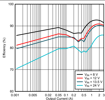
Figure 9-4. LM61430-Q1 Efficiency
