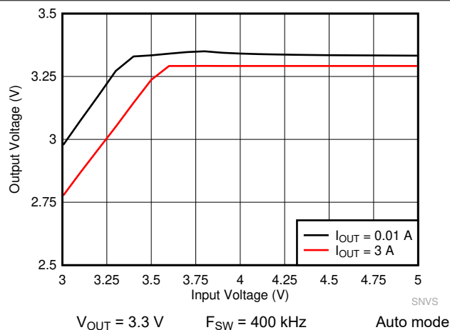
Figure 9-20. LM61430-Q1 Dropout Curve
