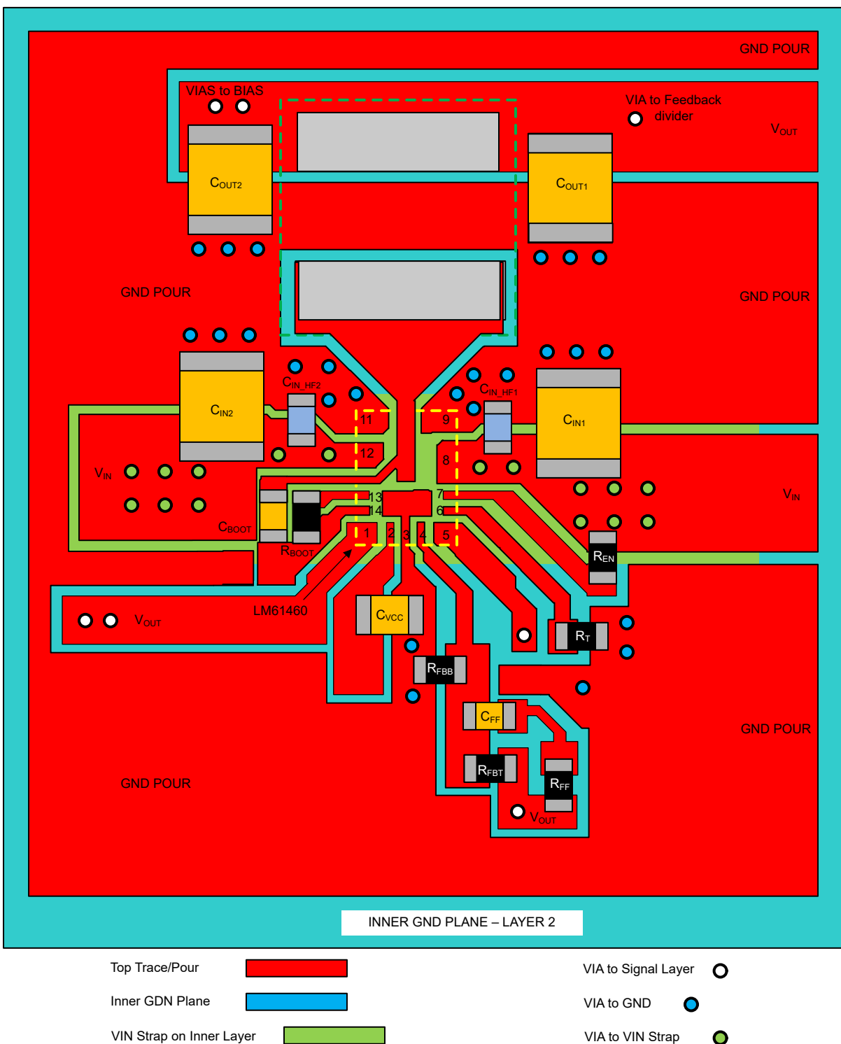
11-2. Layout Example
