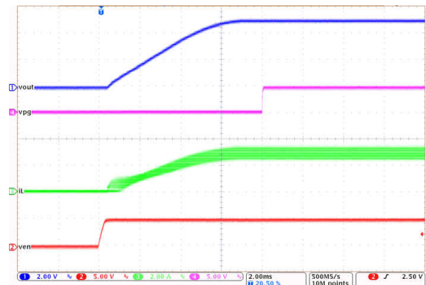
图 9-33. LM61430-Q1 Start-up with 3 A
