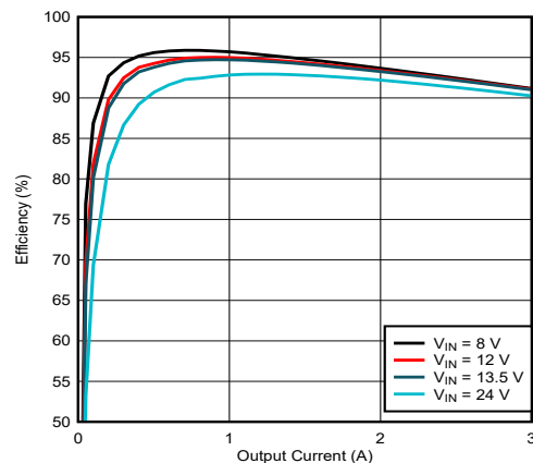
Figure 9-5. LM61430-Q1 Efficiency
