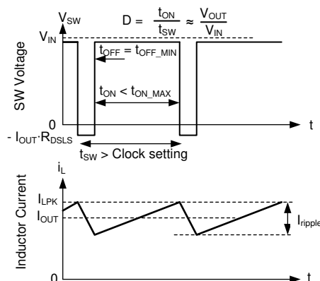
8-19. Frequency and Output Voltage in Dropout
