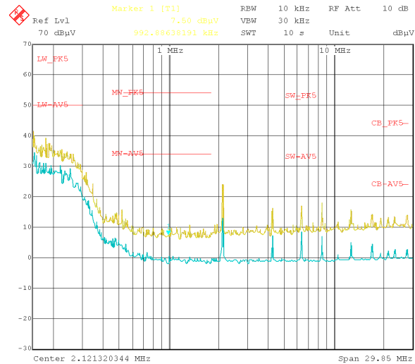
Figure 9-44. Radiated EMI Log Horizontal Versus CISPR25 Limits
