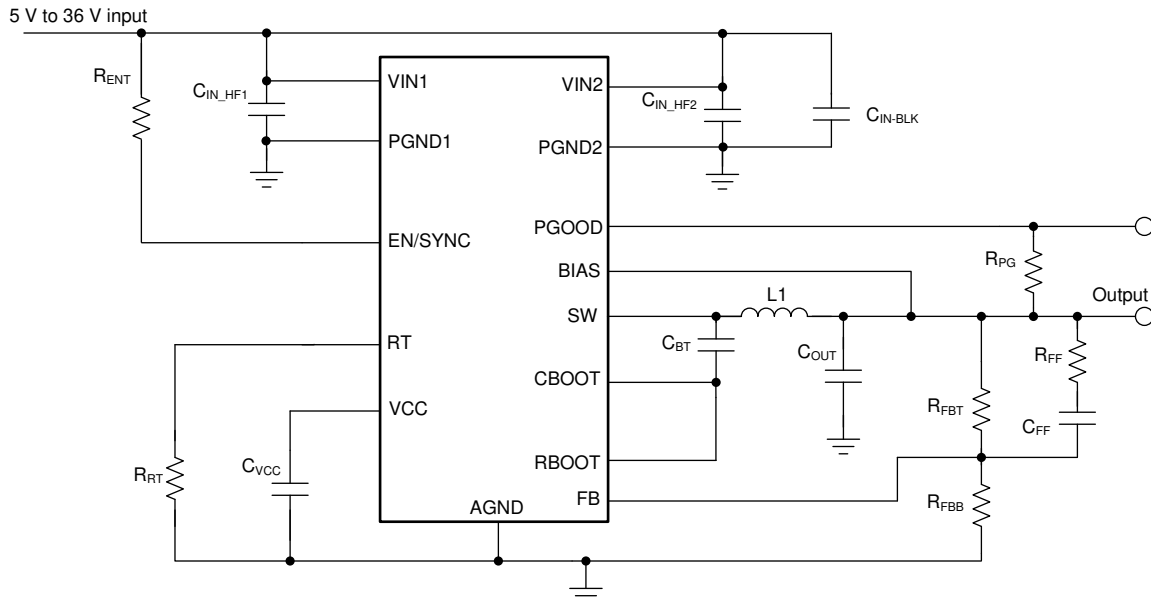
図 9-1. Example Application Circuit
