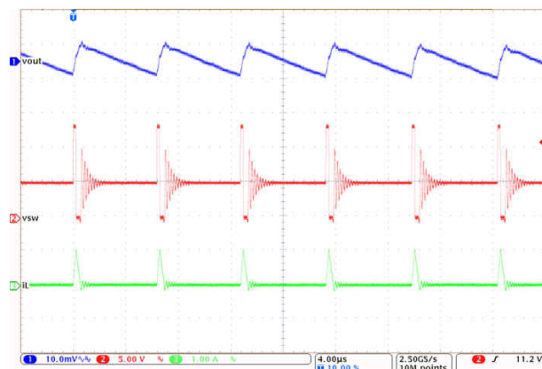
Figure 9-28. LM61430-Q1 Switching Waveform and V_{OUT} Ripple
