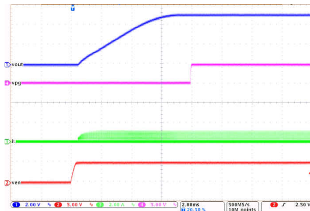
图 9-32. LM61430-Q1 Start-up with 100-mA Load
