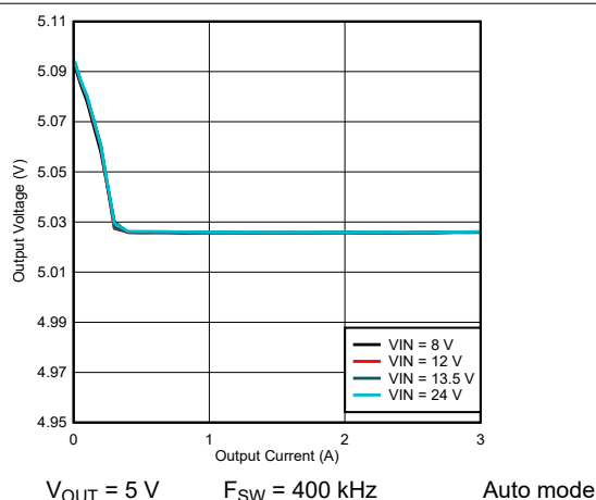
Figure 9-16. LM61430-Q1 Load and Line Regulation
