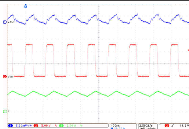
Figure 9-28. LM61430-Q1 Switching Waveform and V_{OUT} Ripple
