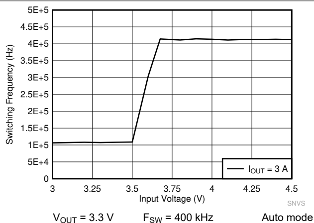
Figure 9-24. LM61430-Q1 Frequency Dropout Curve
