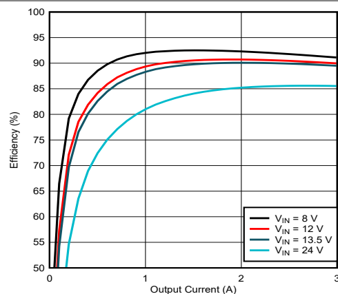
Figure 9-5. LM61430-Q1 Efficiency
