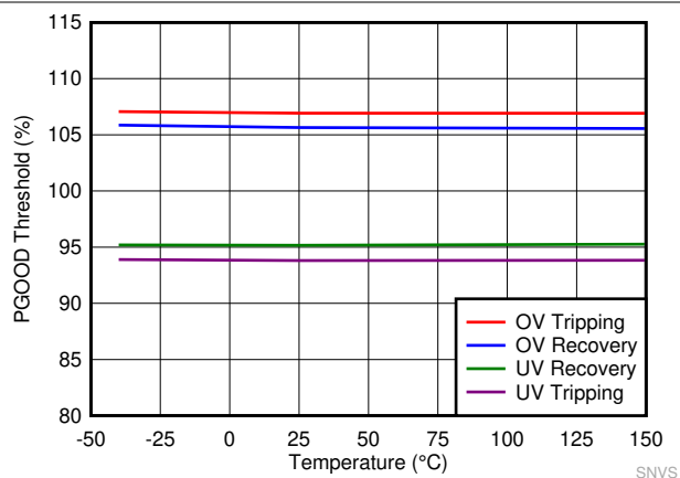
7-7. PGOOD Thresholds
