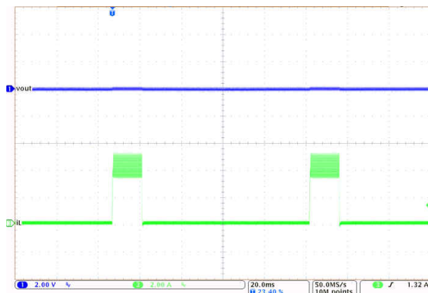
8-12. Inductor Current Bursts During Hiccup
