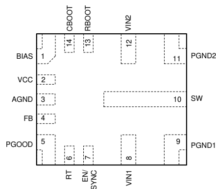
図 6-1. RJR Package 14-Pin VQFN-HR (Top View)
