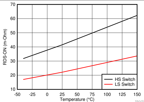
7-5. High-Side and Low-Side Switches R_{DS\_ON}
