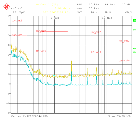
伝導 EMI : V OUT = 5V、F SW = 2100kHz
