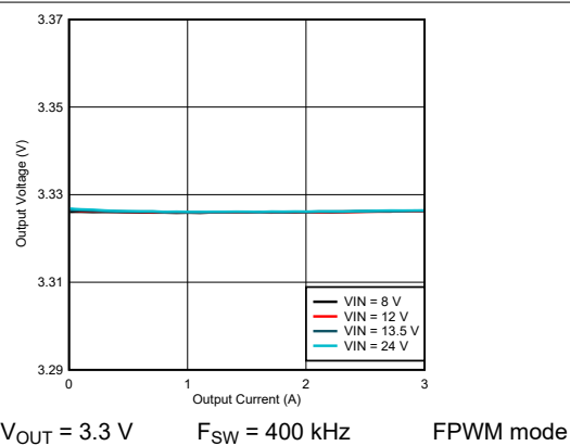
Figure 9-13. LM61430-Q1 Load and Line Regulation
