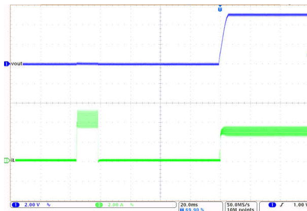
8-13. Short-Circuit Recovery
