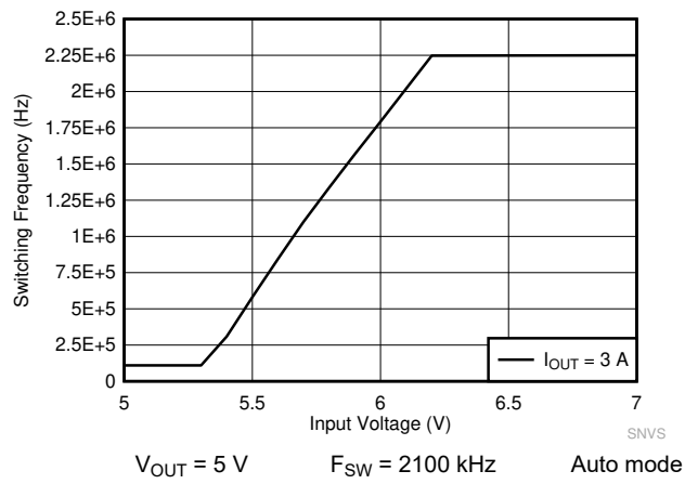
Figure 9-27. LM61430-Q1 Frequency Dropout Curve
