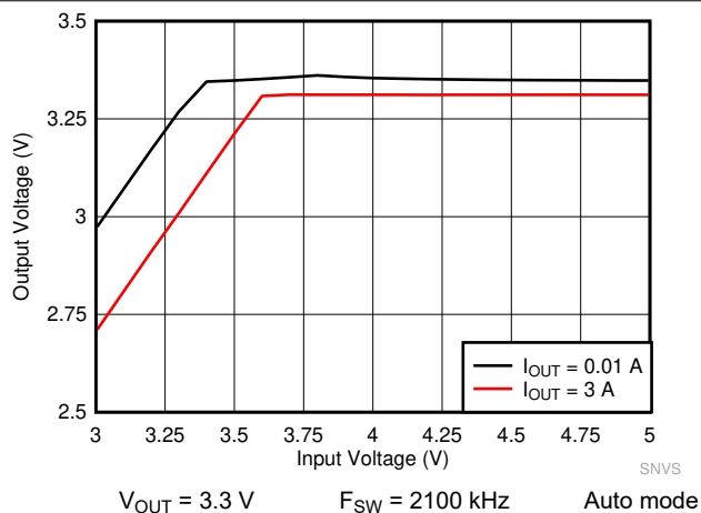
Figure 9-21. LM61430-Q1 Dropout Curve
