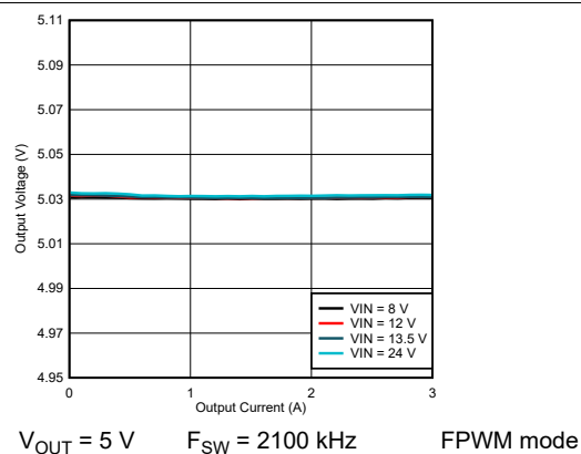
Figure 9-19. LM61430-Q1 Load and Line Regulation
