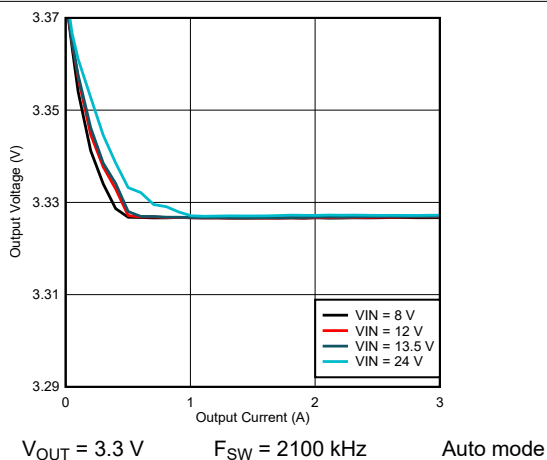
Figure 9-14. LM61430-Q1 Load and Line Regulation
