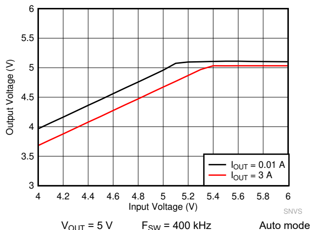
Figure 9-22. LM61430-Q1 Dropout Curve
