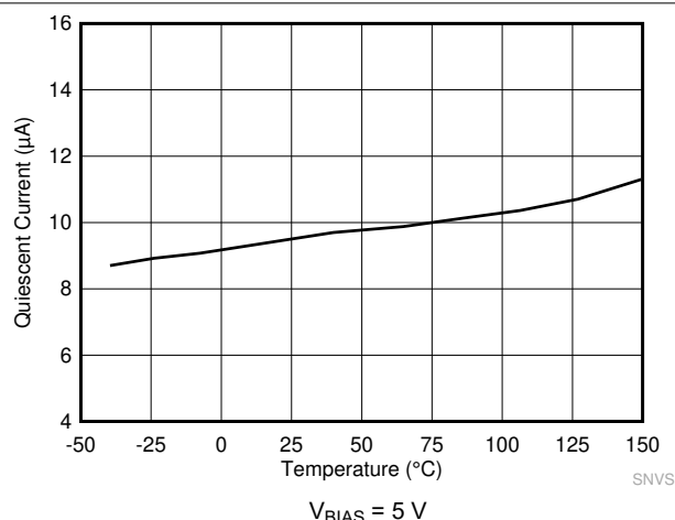
7-1. Nonswitching Input Supply Current
