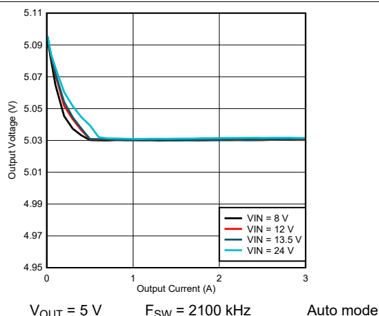
Figure 9-18. LM61430-Q1 Load and Line Regulation
