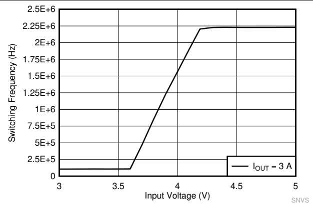
图 9-20. LM61435-Q1 Dropout Curve
