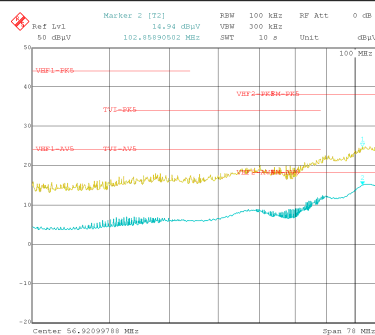
FIG 10-47. Conducted EMI versus CISPR25 Limits (Yellow: Peak Signal, Blue: Average Signal)
