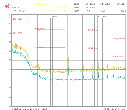
图 10-54. Conducted EMI versus CISPR25 Limits (Yellow: Peak Signal, Blue: Average Signal)
