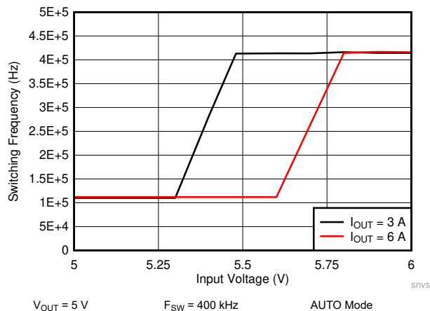
图 10-27. LM61460-Q1 Frequency Dropout Curve
