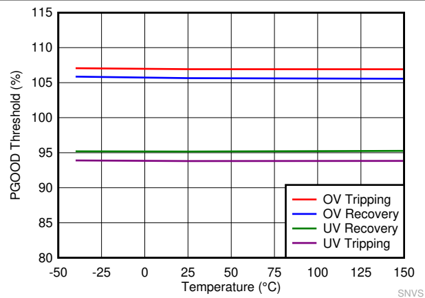
图 8-8. PGOOD Thresholds
