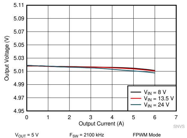
图 10-20. LM61460-Q1 Load and Line Regulation
