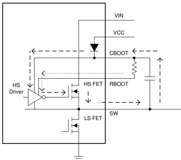
FIG 9-7. Simplified Circuit Showing How RBOOT Functions
