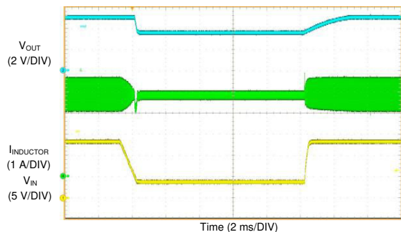
FIG 10-35. LM61460-Q1 Short Circuit Recovery
