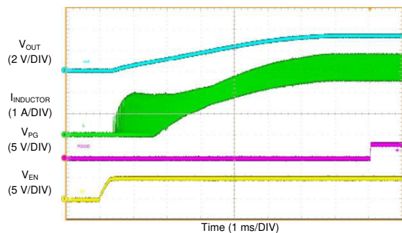
FIG 10-31. LM61460-Q1 Start-up with 50-mA Load
