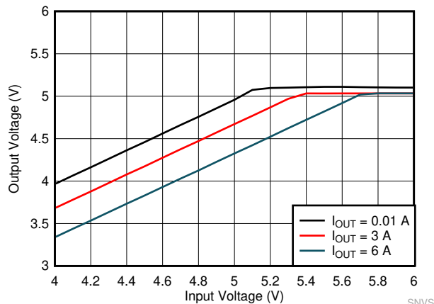
图 10-23. Dropout Curve
