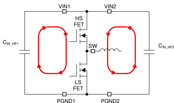
FIG 12-1. Input Current Loop
