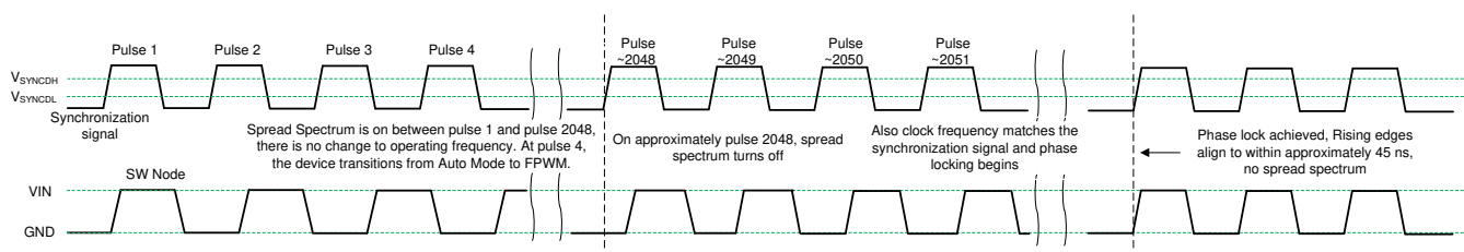
FIG 9-4. Synchronization Process
