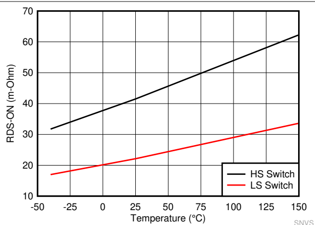
Figure 8-6. High-side and Low-side Switches R_{DS\_ON}
