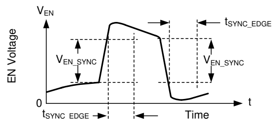
FIG 9-3. Typical SYNC/EN Waveform
