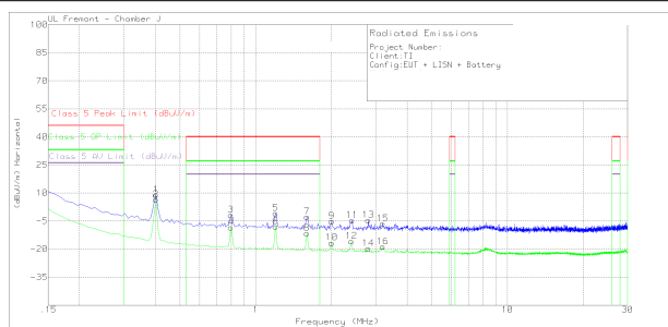
FIG 10-48. Radiated EMI Rod versus CISPR25 Limits
