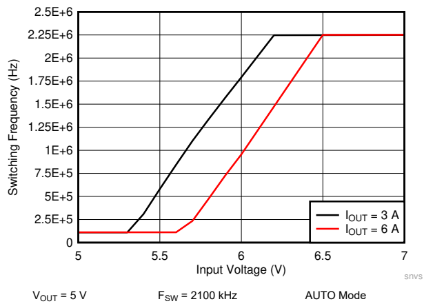
图 10-28. LM61460-Q1 Frequency Dropout Curve
