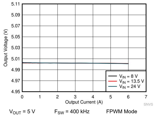
图 10-18. LM61460-Q1 Load and Line Regulation
