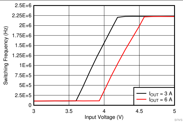
图 10-26. LM61460-Q1 Frequency Dropout Curve
