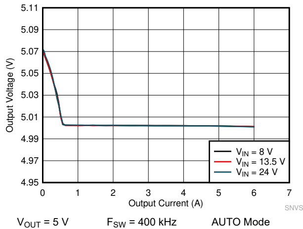
图 10-17. LM61460-Q1 Load and Line Regulation
