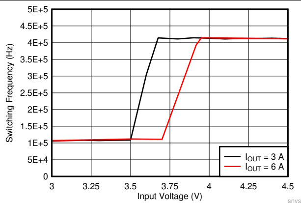
图 10-23. Dropout Curve
