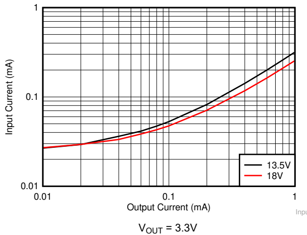
8-15. Input Supply Current versus Output Current
