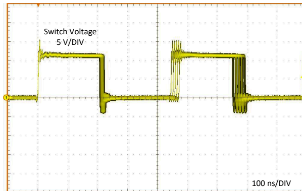
図 7-7. Typical PWM Switching Waveforms With Spread Spectrum V_{IN} = 12V , V_{OUT} = 5V , I_{OUT} = 2.5A , f_{SW} = 2100kHz
