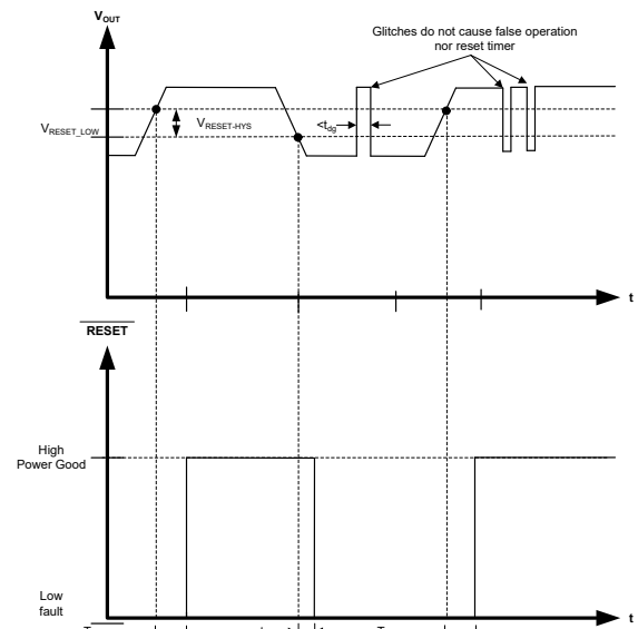
図 7-4. RESET Timing Behavior
