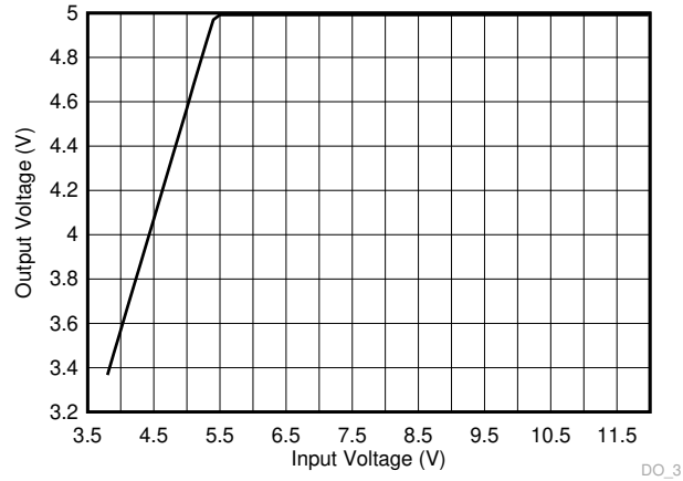
図 7-8. Overall Dropout Characteristic V_{OUT} = 5V , I_{OUT} = 3.25A
