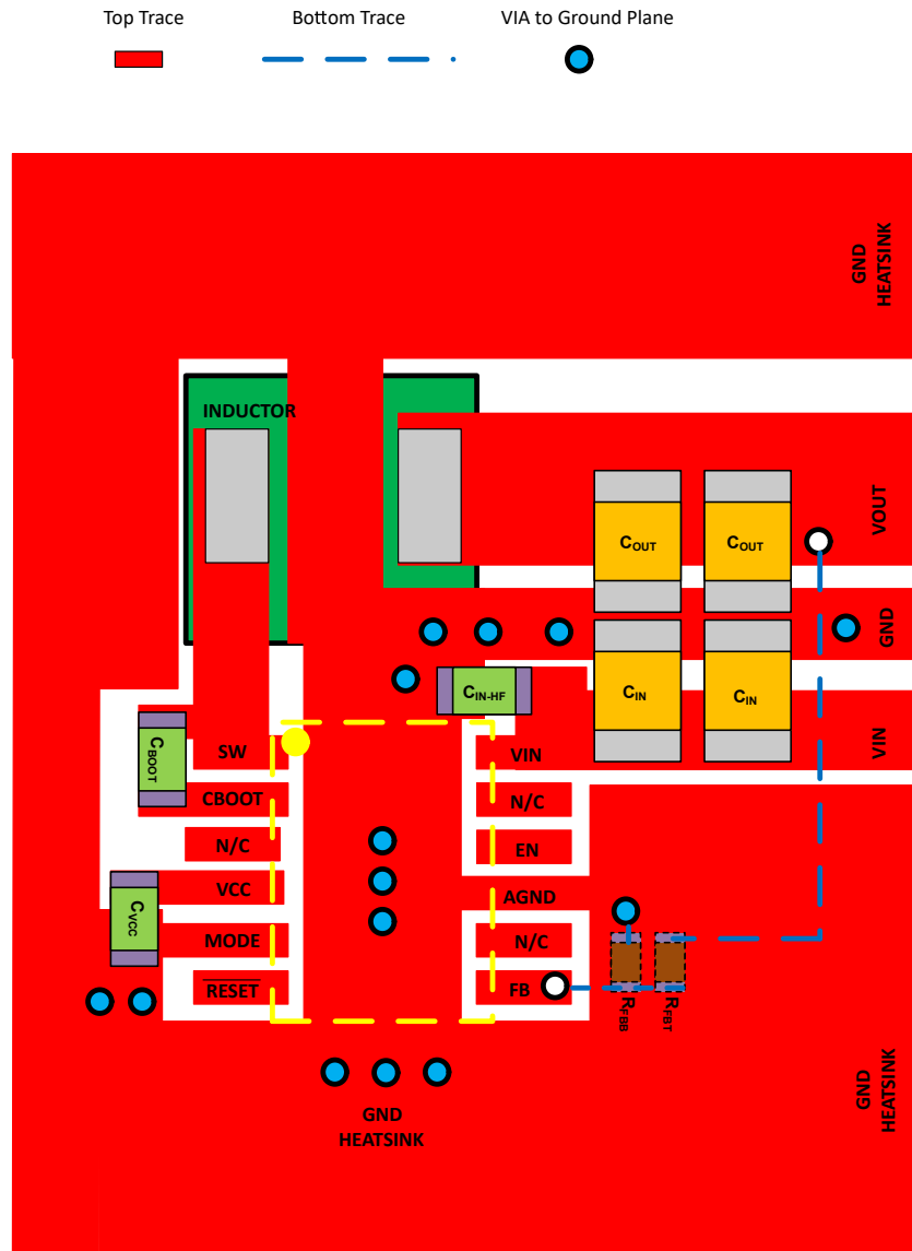
図 8-20. Example Layout for WSON Package
