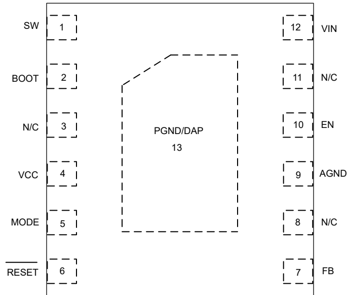
図 5-1. DRR Package, 12-Pin WSON With PowerPAD™ Integrated Circuit Package— LM63635C-Q1 (Top View)
