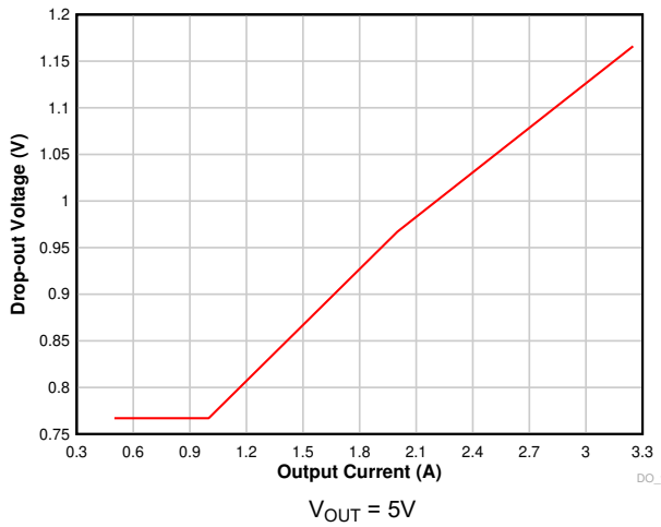
8-13. Dropout Voltage versus Output Current to 1.85MHz
