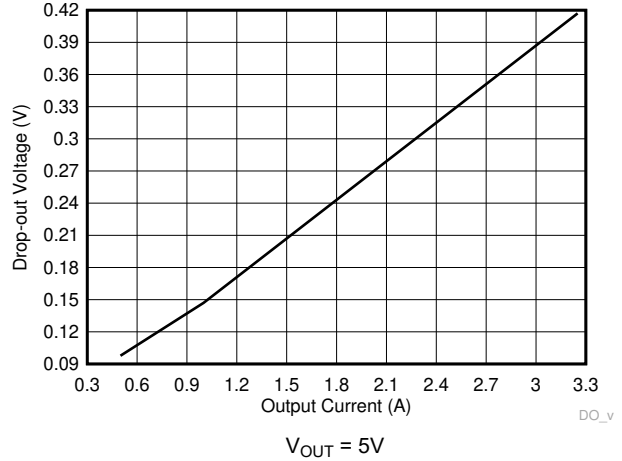
8-12. Dropout Voltage versus Output Current for -1% Drop
