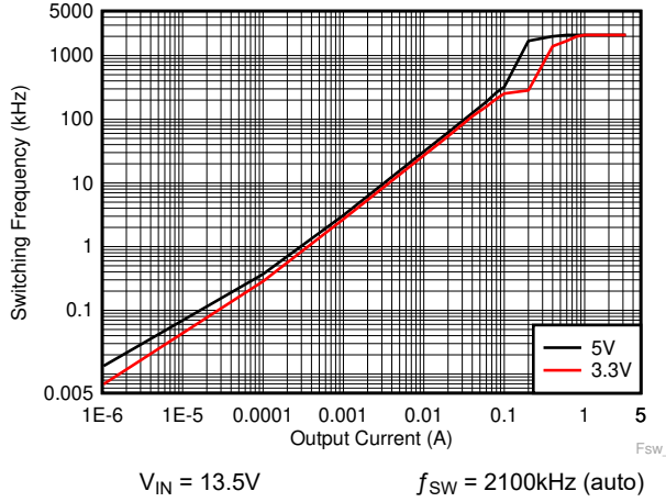
8-11. Switching Frequency versus Output Current
