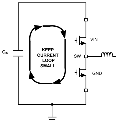
图 8-19. Current Loops With Fast Edges
