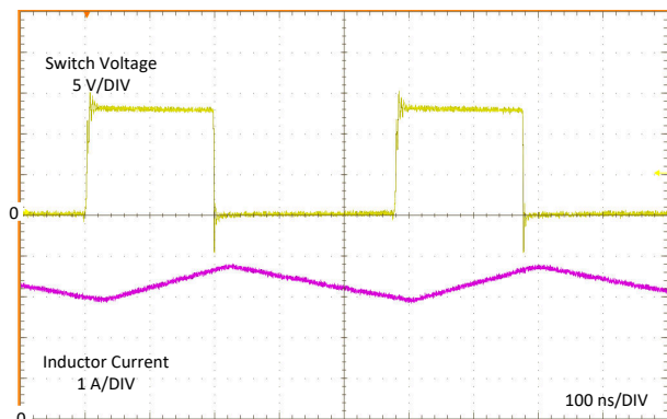
図 7-6. Typical PWM Switching Waveforms Without Spread Spectrum V_{IN} = 12V , V_{OUT} = 5V , I_{OUT} = 3.25A , f_{SW} = 2100kHz
