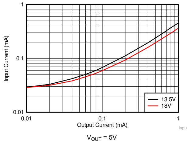
8-14. Input Supply Current versus Output Current
