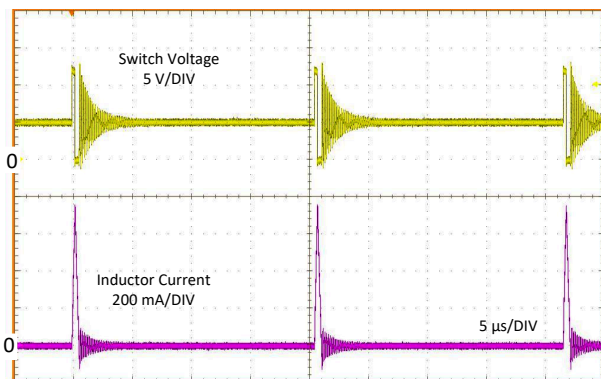
図 7-5. Typical PFM Switching Waveforms V_{IN} = 12V , V_{OUT} = 5V , I_{OUT} = 10mA
