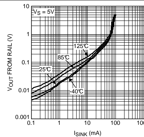
Figure 18. Output Swing vs Sinking Current
