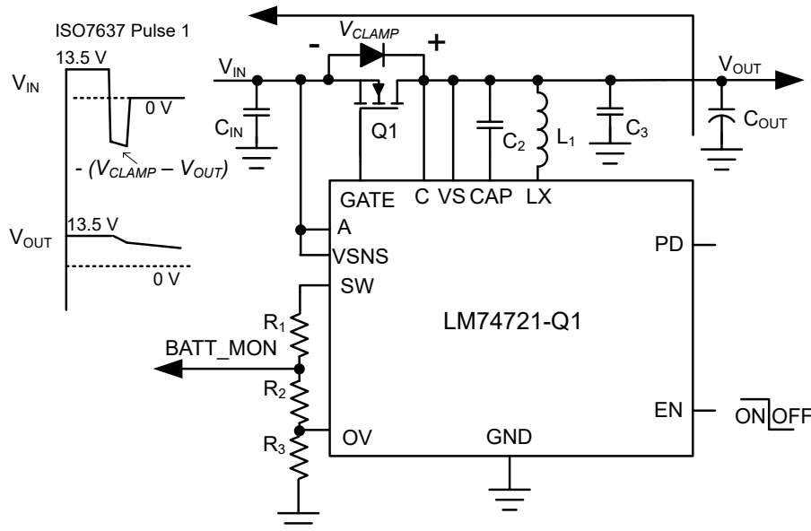
FIG 8-2. LM74721-Q1 Ideal Diode Circuit Operation During ISO7637 Pulse 1
