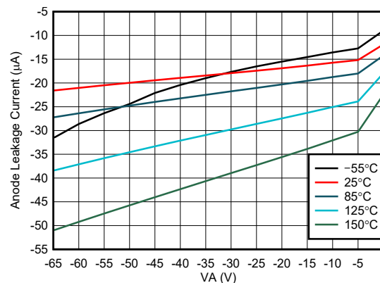
图 6-8. ANODE Leakage Current vs Reverse ANODE Voltage
