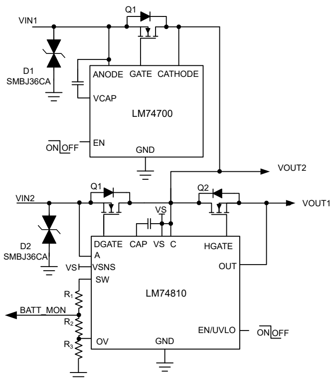
8-5. Redundant Supply OR-ing With Overvoltage Protection and ON/OFF Control
