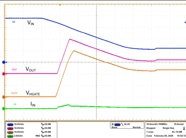
Figure 9-7. Overvoltage Recovery
