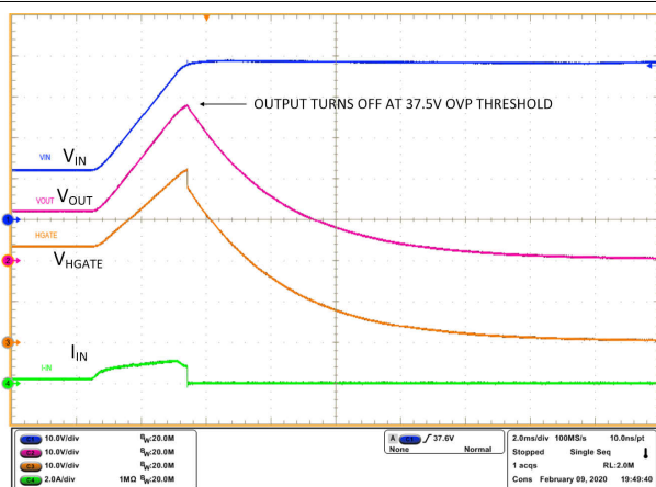
Figure 9-6. Overvoltage Cut-off
