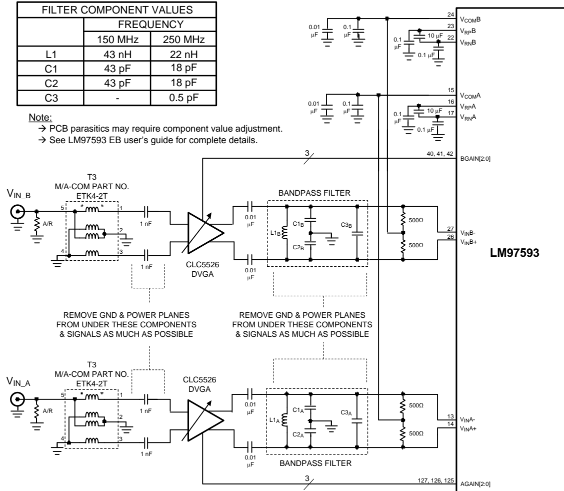
Figure 86. Application Circuit
