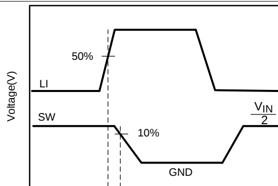
FIG 7. Low-Side Gate Driver Turnon
