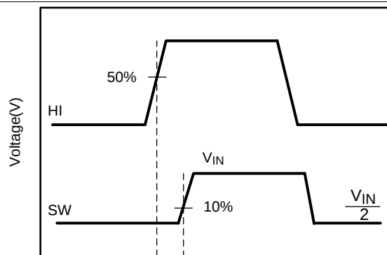
FIG 6. High-Side Gate Driver Turnon
