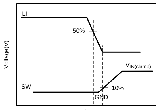
FIG 9. Low-Side Gate Driver Turnoff
