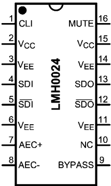
16-Pin SOIC Order Number LMH0024MA See NS Package Number M16A
