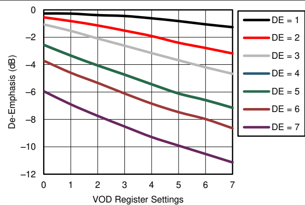
FIG 7-7. OUT0 De-Emphasis vs. OUT0 VOD and DE Register Settings
