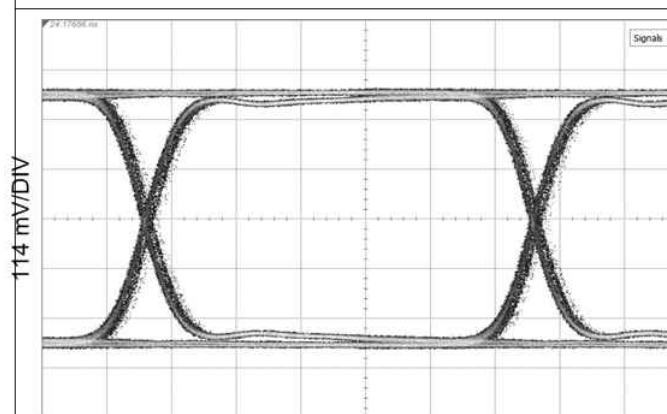
FIG 9-7. 5.94 Gbps, CC = 120-m Belden 1694A, Reclocked
