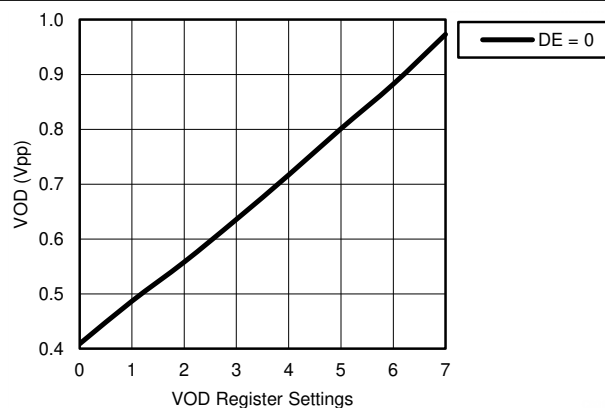
FIG 7-6. OUT0 VOD vs. OUT0 VOD and DE Register Settings
