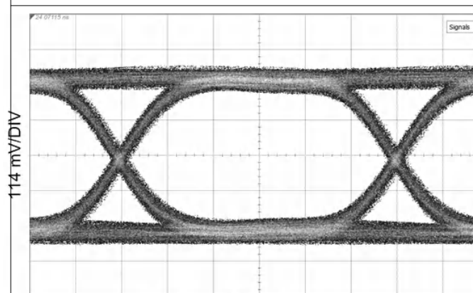
FIG 9-5. 11.88 Gbps, CC = 75-m Belden 1694A, Reclocked
