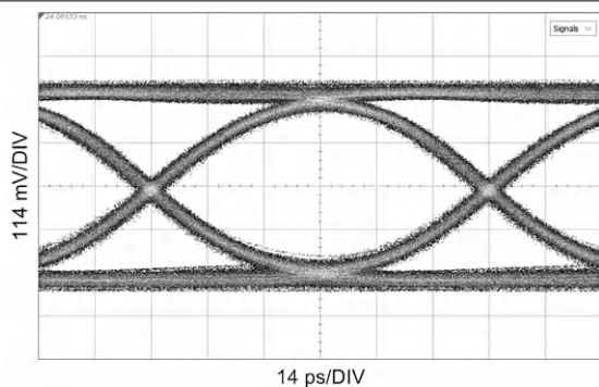
FIG 7-4. EQ Mode at 11.88 Gbps, Measured at OUT0±, 75-m Belden 1694A Before SDI_IO+
