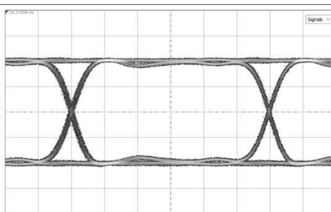
FIG 9-8. 5.94 Gbps, TL = 20" FR4, Reclocked
