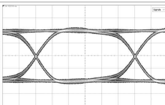
FIG 9-6. 11.88 Gbps, TL = 20" FR4, Reclocked
